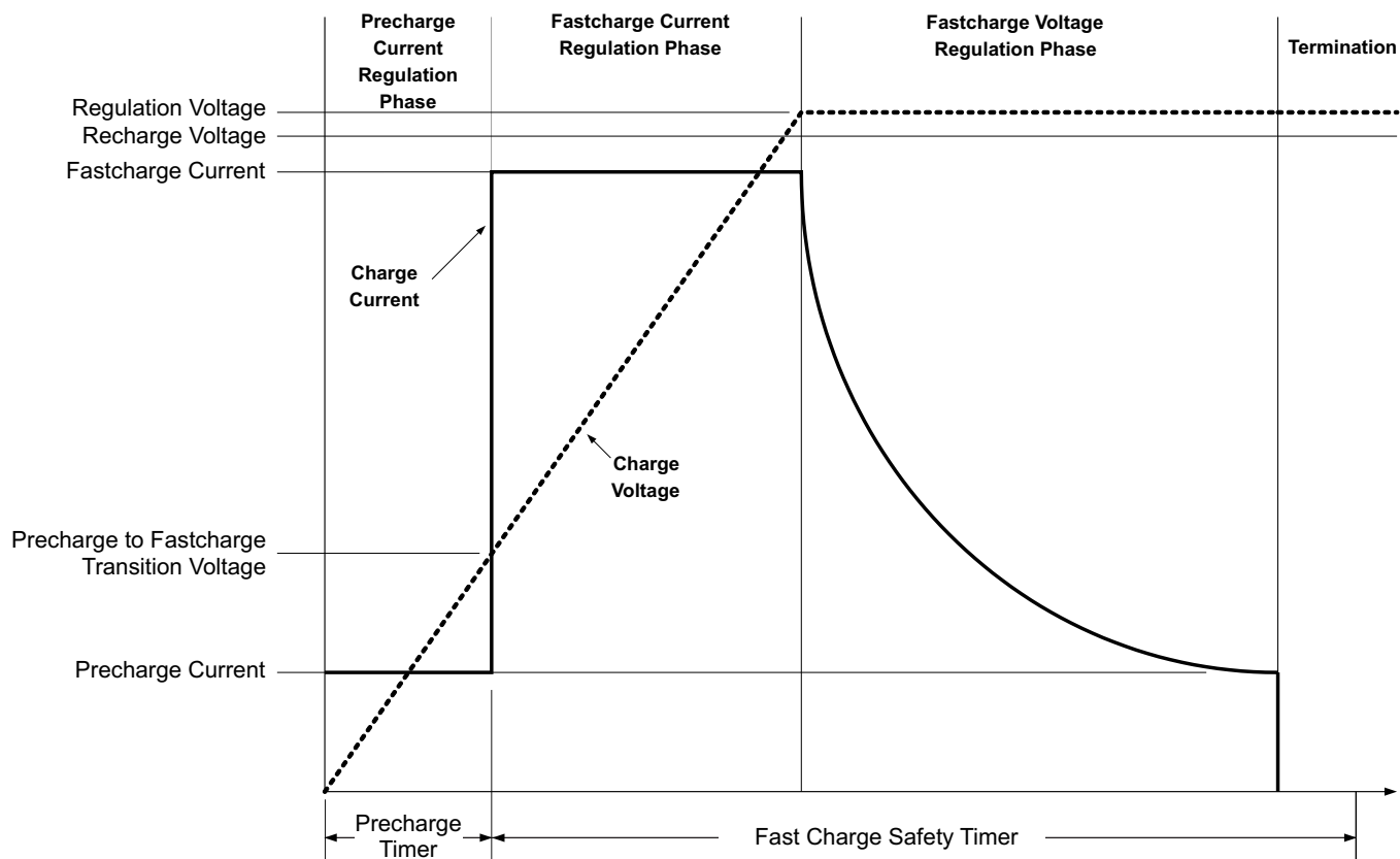
Figure 3-8. Charging Cycle
