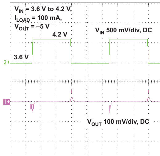
t - Time - 2 ms/div
