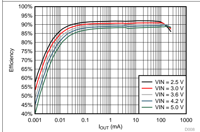
Figure 7. Efficiency vs Load Current, V_{OUT} = 3.3\text{ V}
