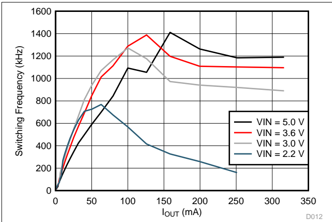
Figure 13. Switching Frequency vs Load Current V OUT = 1.8 V
