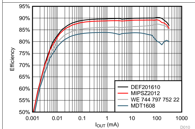
Figure 9. Efficiency vs Load Current; V_{OUT} = 1.8\text{ V}
