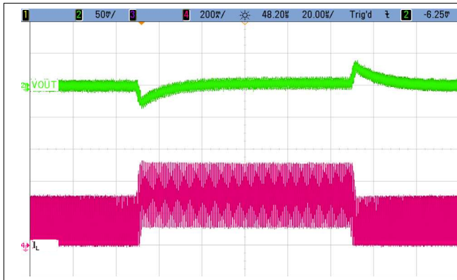
Figure 19. Load Transient Response; 100 mA to 290 mA
