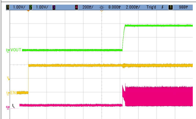
Figure 15. PFM (Power Save Mode) Mode Operation
