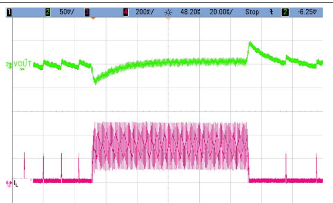
Figure 20. Load Transient Response; 5 mA to 290 mA
