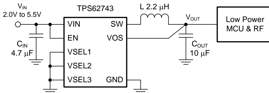
Figure 6. TPS62743 Typical Application Circuit
