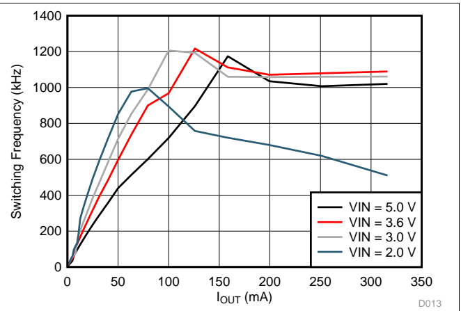
Figure 14. Switching Frequency vs Load Current V OUT = 1.2 V
