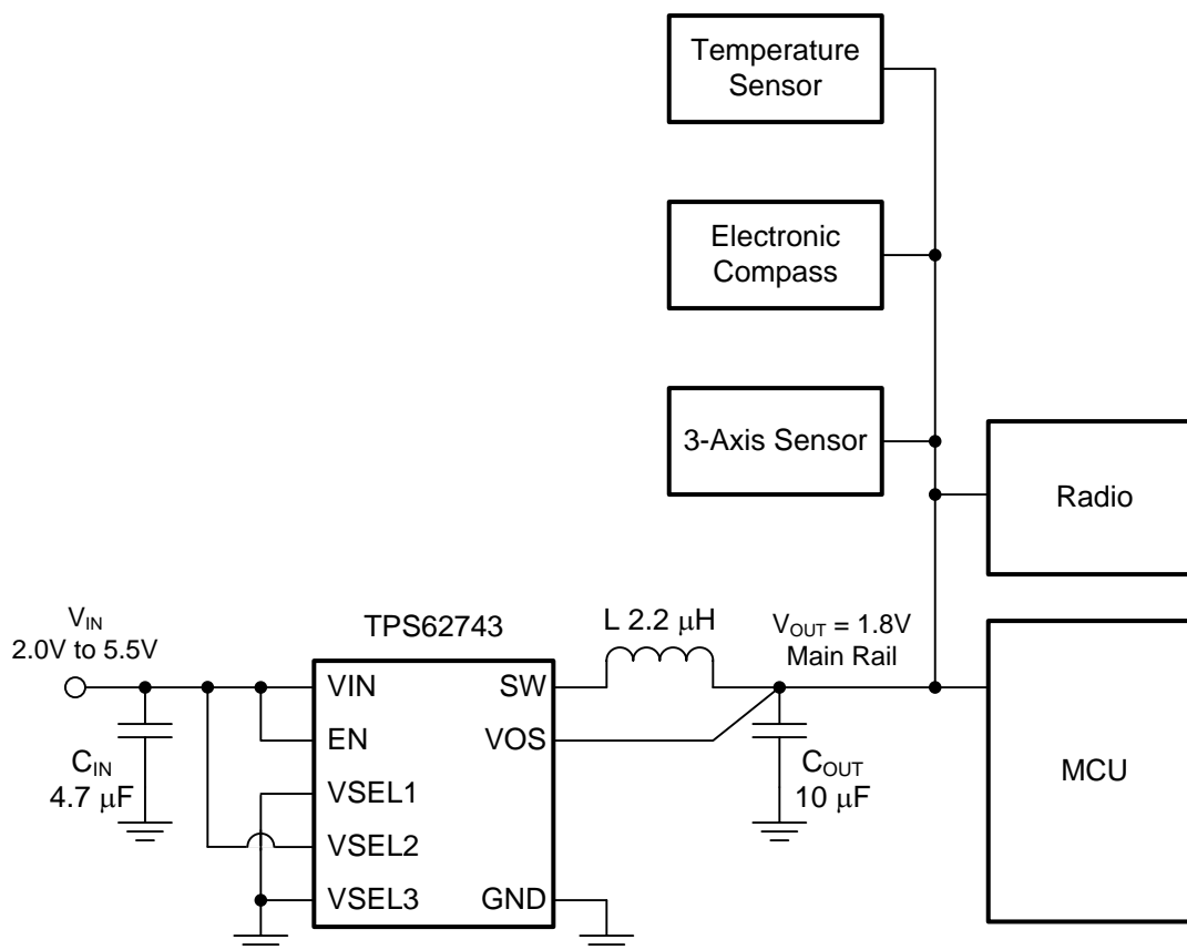
Figure 22. Example Of Implementation In A Master MCU Based System
