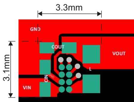
Figure 23. Recommended PCB Layout
