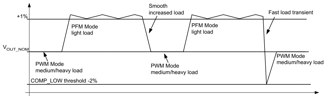
Figure 32. Dynamic Voltage Positioning
