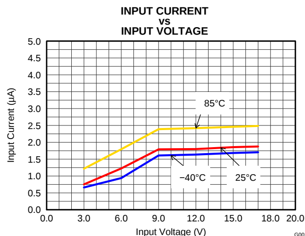
Figure 22. Shutdown Current
