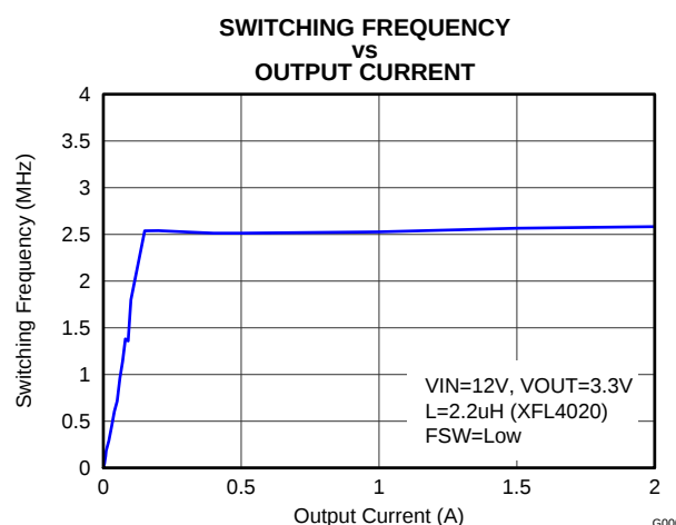
Figure 20. Switching Frequency
