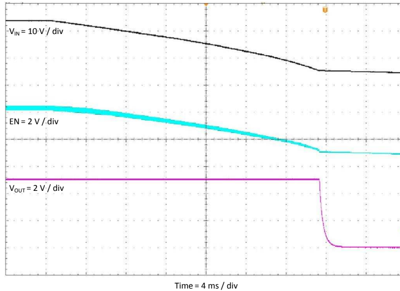
Figure 13. TPS54302EVM-716 Shutdown Relative to V_{IN}
