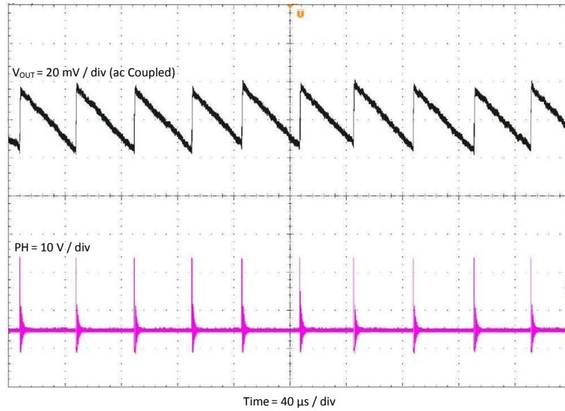
Figure 8. TPS54302EVM-716 Output Ripple, I_{OUT} = 10 \text{ mA}
