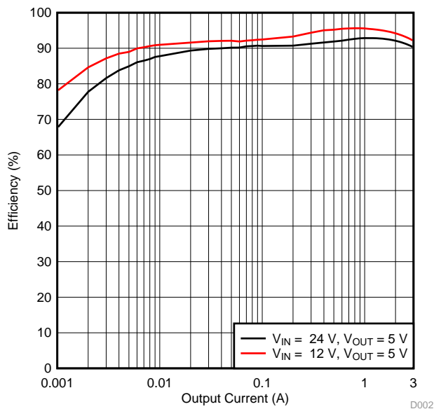
Figure 2. TPS54302EVM-716 Low Current Efficiency
