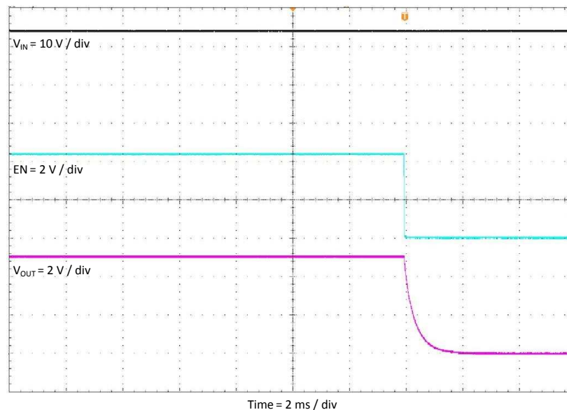
Figure 14. TPS54302EVM-716 Shutdown Relative to EN
