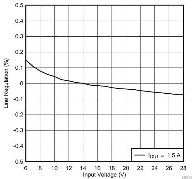
Figure 4. TPS54302EVM-716 Line Regulation
