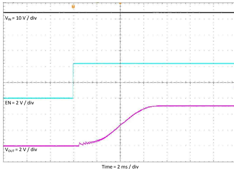
Figure 12. TPS54302EVM-716 Startup Relative to Enable
