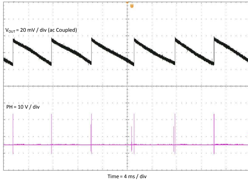
Figure 9. TPS54302EVM-716 Output Ripple, I_{OUT} = 0 \text{ A}
