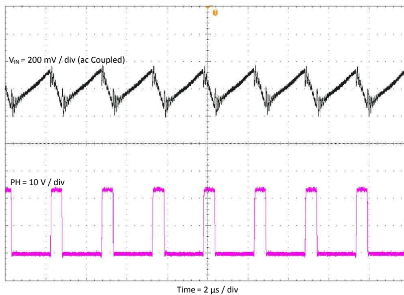
Figure 10. TPS54302EVM-716 Input Ripple
