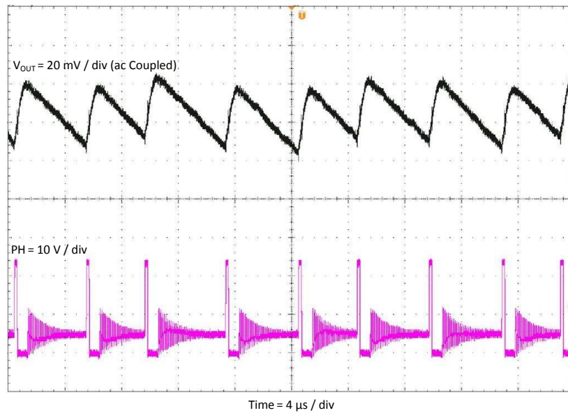
Figure 7. TPS54302EVM-716 Output Ripple, I_{OUT} = 100\text{ mA}
