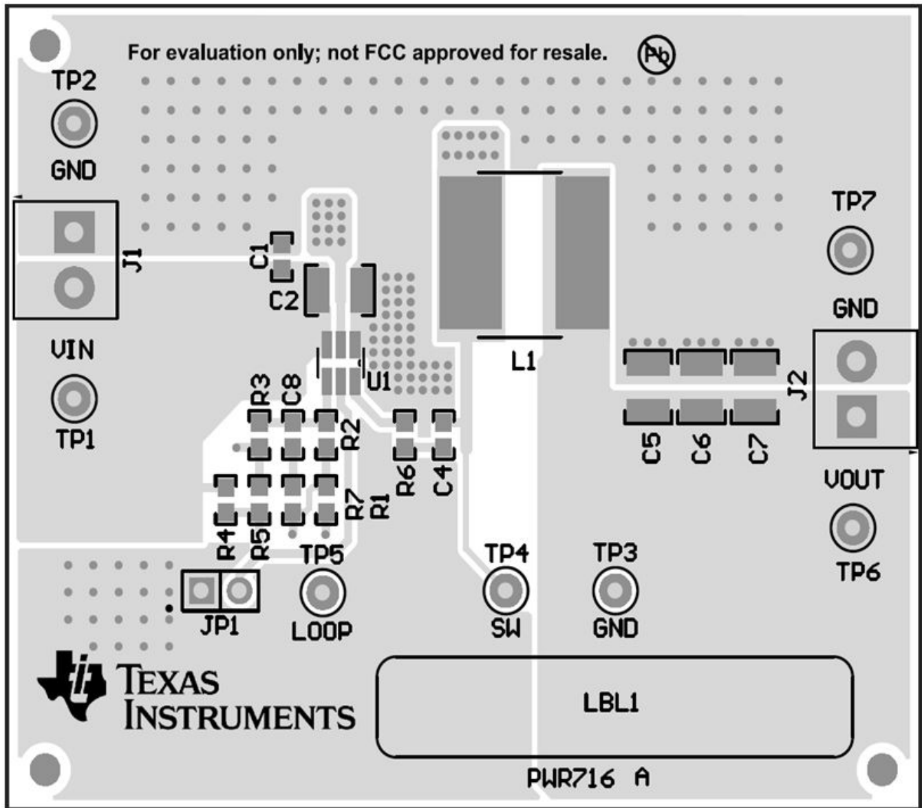
Figure 15. TPS54302EVM-716 Top-Side Assembly
