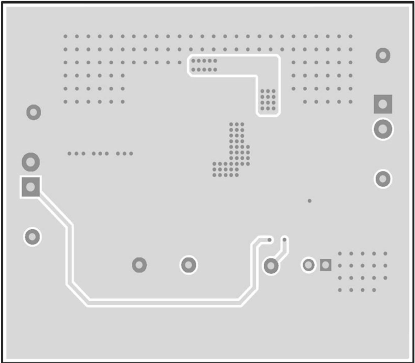
Figure 16. TPS54302EVM-716 Bottom-Side Layout
