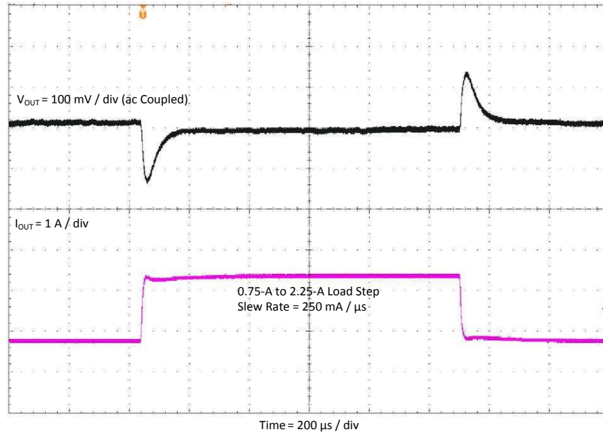
Figure 5. TPS54302EVM-716 Transient Response
