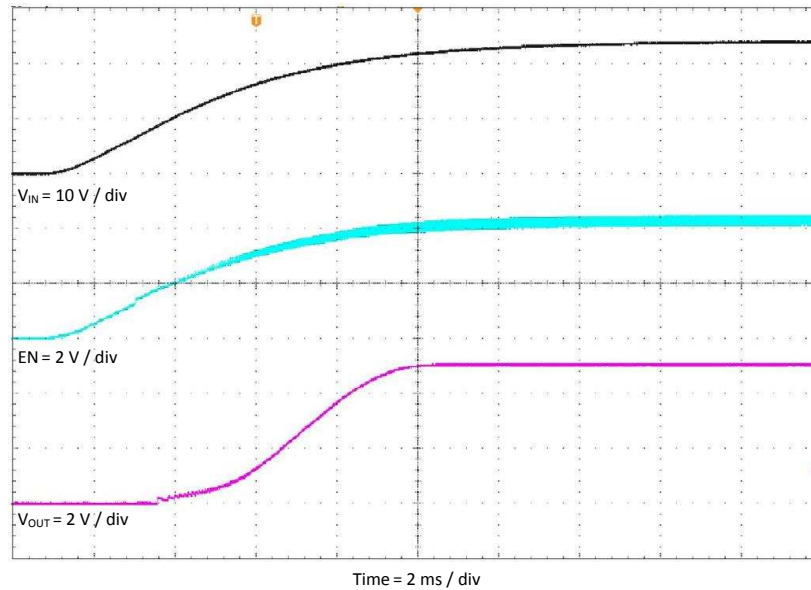
Figure 11. TPS54302EVM-716 Startup Relative to V_{IN}
