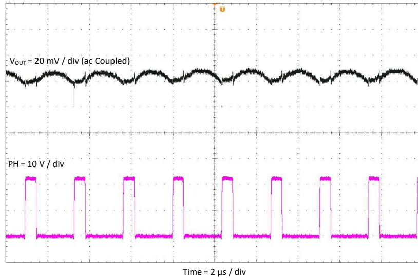
Figure 6. TPS54302EVM-716 Output Ripple, I_{OUT} = 3\text{ A}
