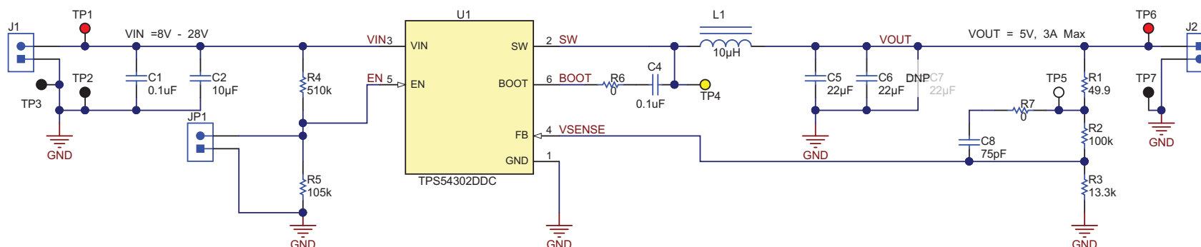
Figure 17. TPS54302EVM-716 Schematic
