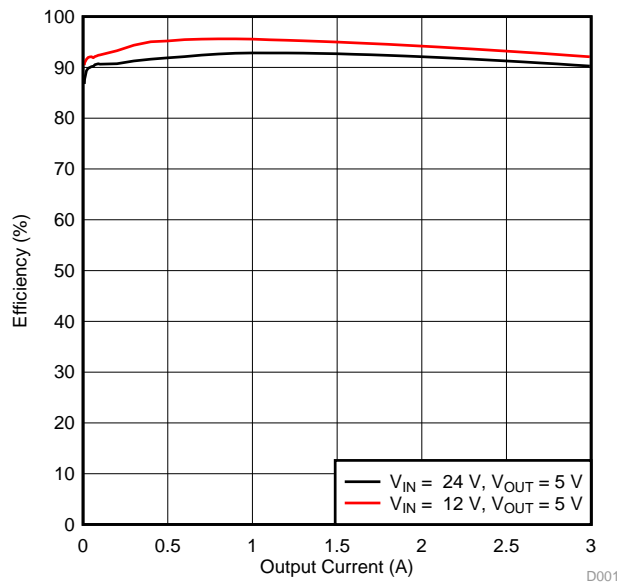
Figure 1. TPS54302EVM-716 Efficiency
