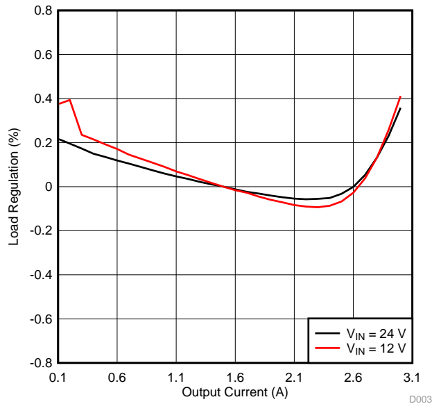
Figure 3. TPS54302EVM-716 Load Regulation
