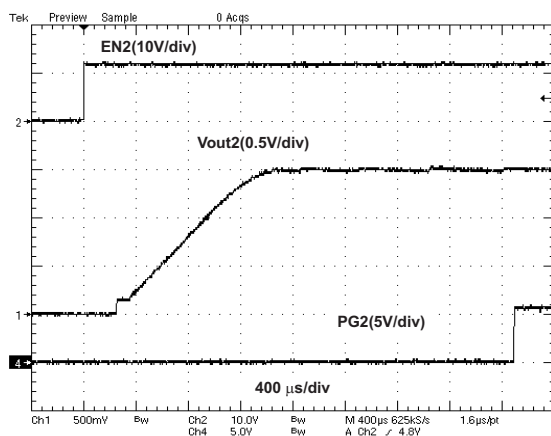
Figure 11. VO2=1.5V, PG2
