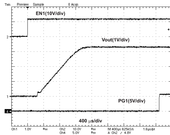
Figure 10. VO1=3.3V, PG1
