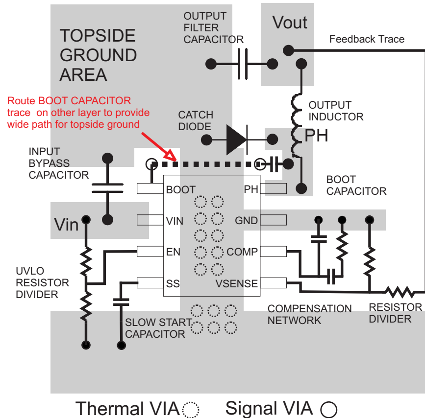
Figure 13. TPS54233 Board Layout
