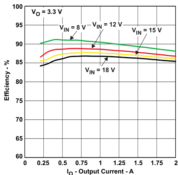
Figure 14. TPS54233 Efficiency
