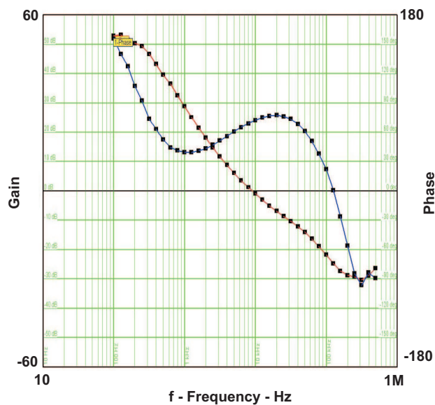
Figure 19. TPS54233 Loop Response
