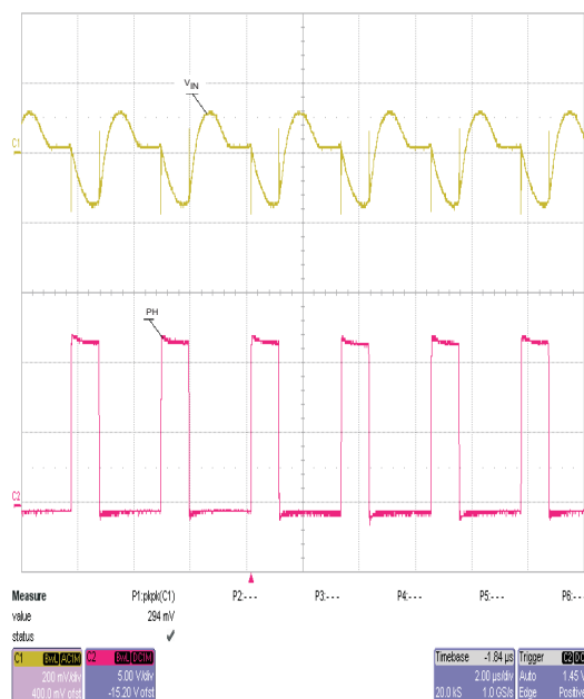
Figure 20. TPS54233 Input Ripple
