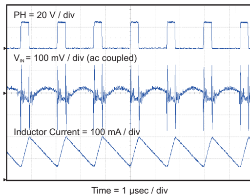
Figure 47. Input Ripple, CCM
