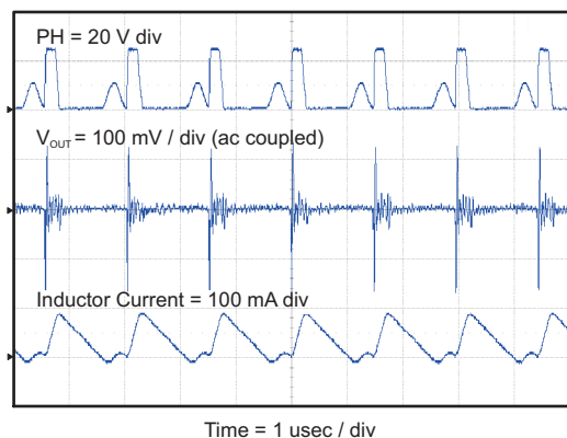
Figure 46. Output Ripple, PSM
