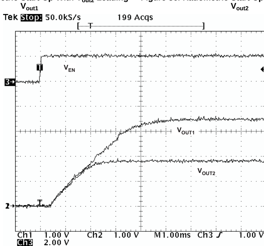
Figure 37. Simultaneous Start-Up
