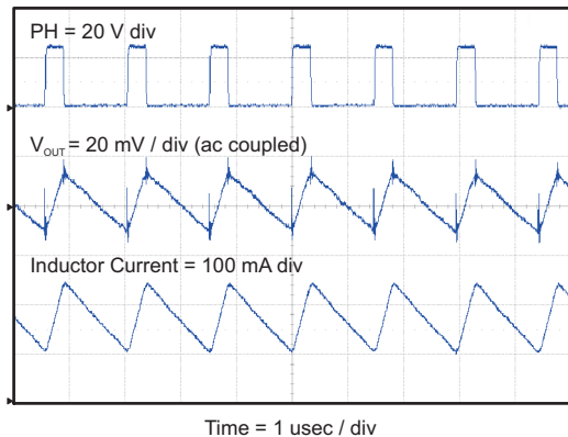
Figure 44. Output Ripple, CCM
