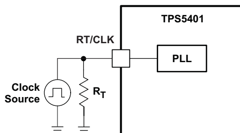
Figure 39. Synchronizing to a System Clock
