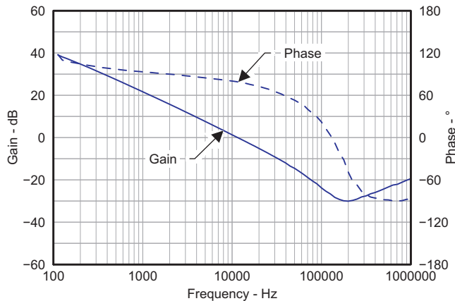
Figure 51. Overall Loop-Frequency Response
