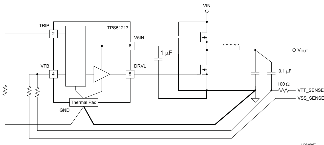
Figure 25. Remote Sensing of Output Voltage Using the TPS51217
