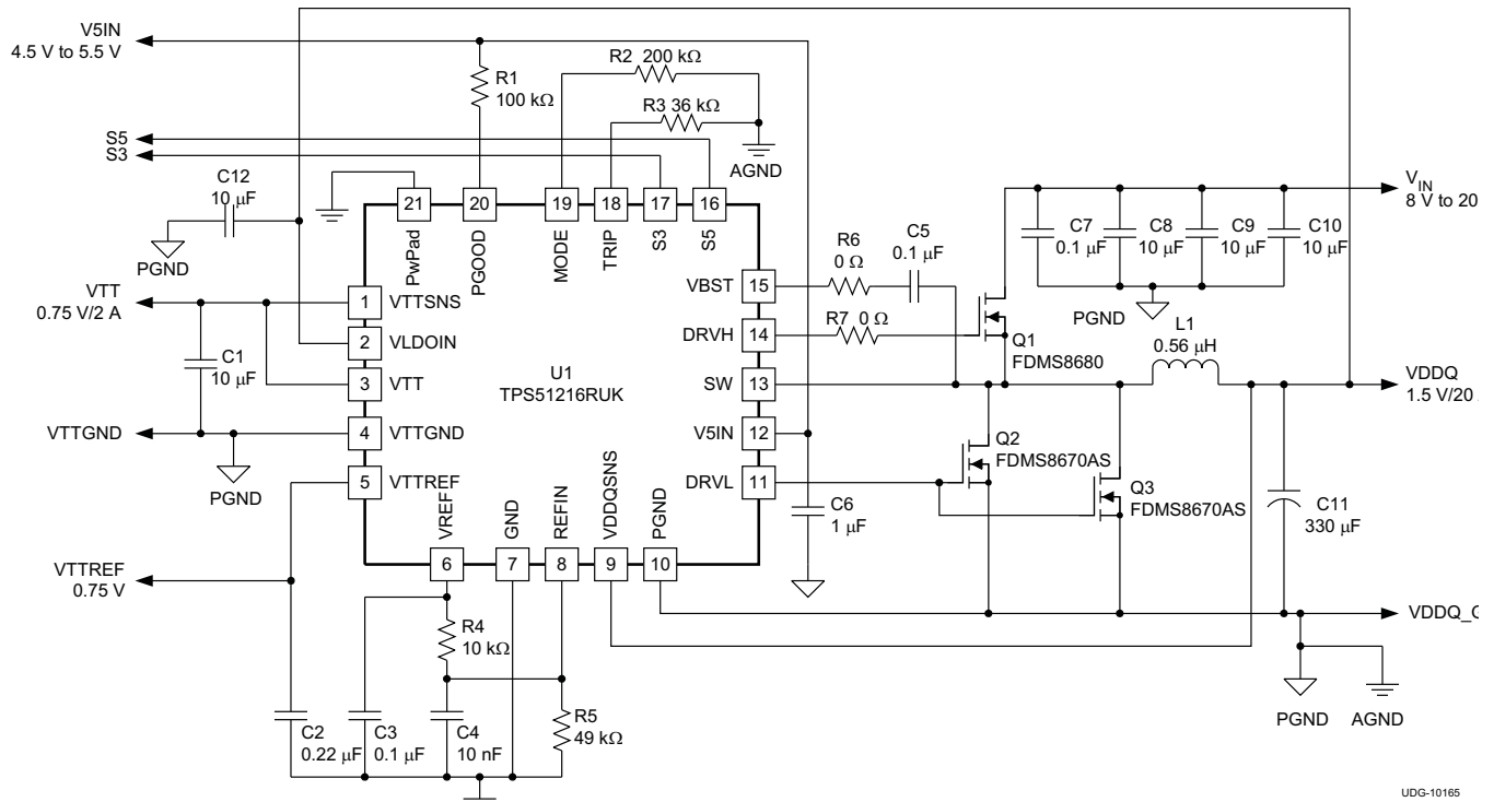
Figure 32. DDR3, 400-kHz Application Circuit, Tracking Discharge
