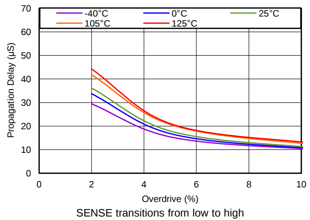
Figure 9. Overvoltage Propagation Delay vs Overdrive
