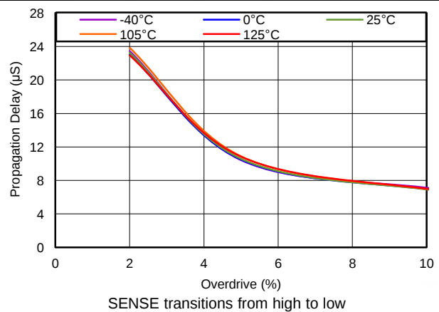
Figure 11. Overvoltage Propagation Delay vs Overdrive
