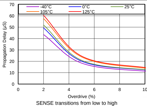
Figure 10. Undervoltage Propagation Delay vs Overdrive
