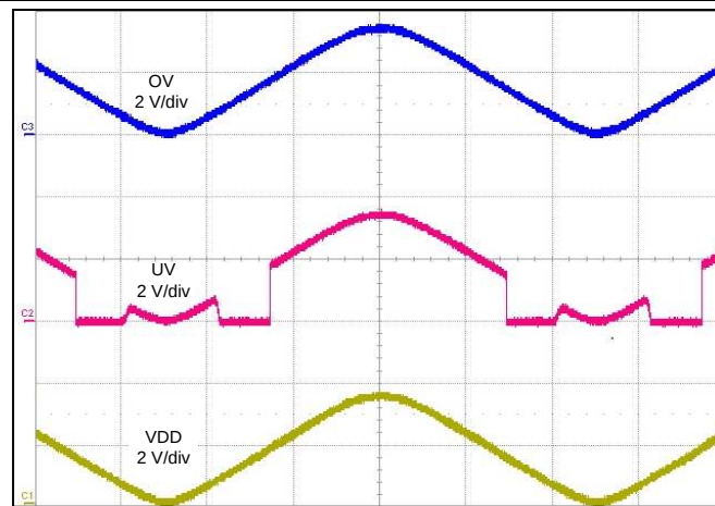
Figure 23. TPS3702CX33 Startup with V_{\text{PULLUP}} = 3 V
