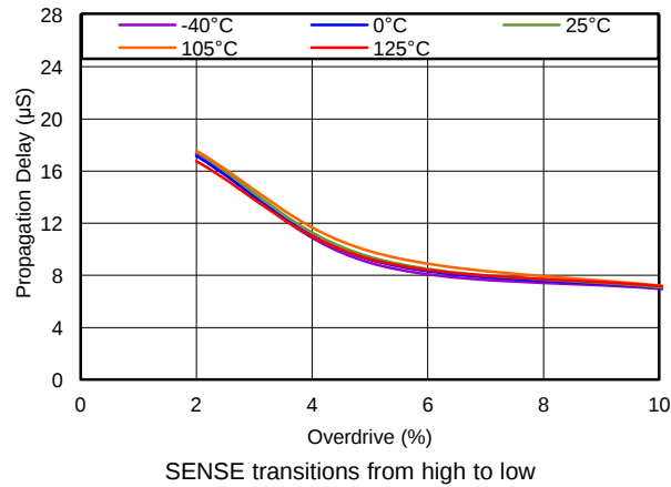
Figure 8. Undervoltage Propagation Delay vs Overdrive
