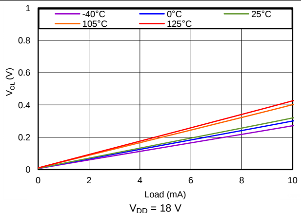
Figure 13. Low-Level Output Voltage vs Output Current
