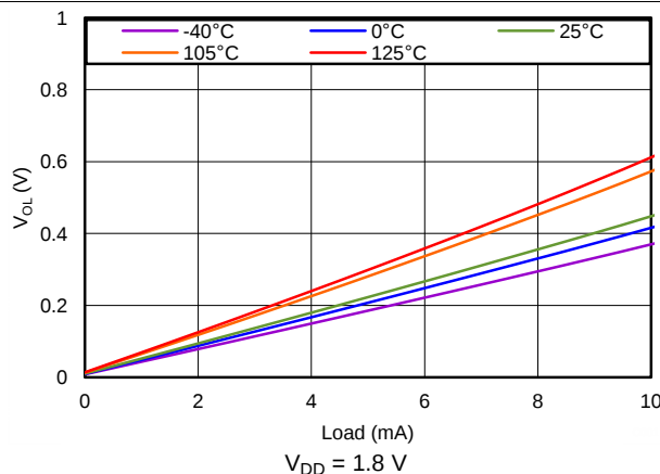
Figure 12. Low-Level Output Voltage vs Output Current
