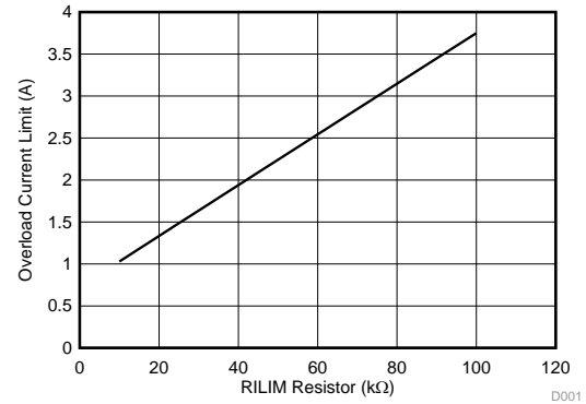
Figure 32. I_{\text{RILIM}} Resistor vs Overload Current Limit
