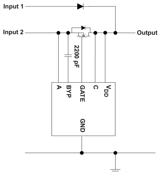
Figure 19. ORing Circuit
