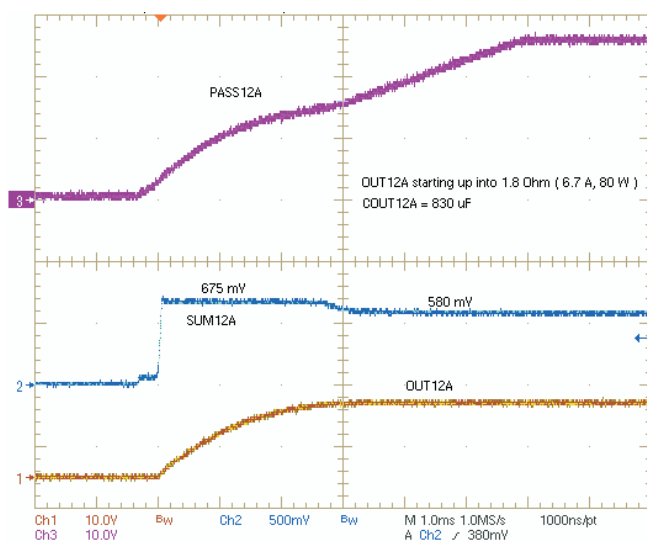
Figure 18. OUT12A Startup Into 80-Watt, 830- \mu F Load
