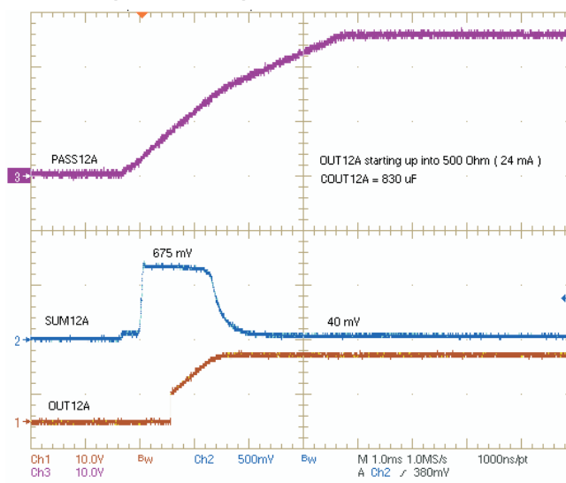
Figure 17. OUT12A Startup Into 500- \Omega , 830- \mu F Load
