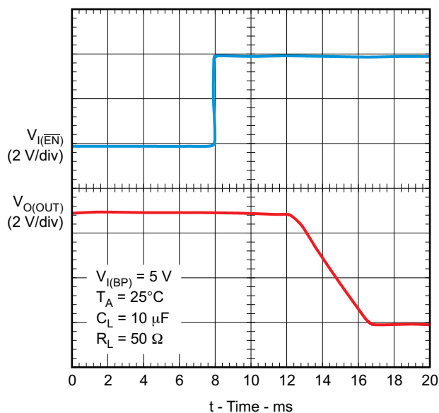
Figure 4. Turnoff Delay and Fall Time (BP Switch)
