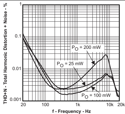
R_L = 32 \Omega BTL V_{DD} = 3.6 V Gain = 6.1 dB
