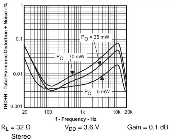
Figure 15. Total Harmonic Distortion + Noise vs Frequency
