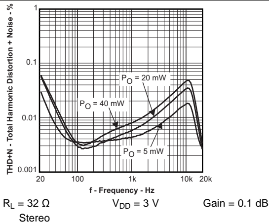
Figure 14. Total Harmonic Distortion + Noise vs Frequency
