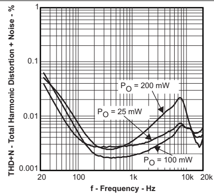
R_L = 32 \Omega BTL V_{DD} = 5 V Gain = 6.1 dB
