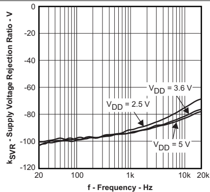
R_L = 16 \Omega Stereo C_p = 1 \mu F Gain = 0.1 dB
