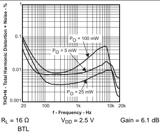
Figure 17. Total Harmonic Distortion + Noise vs Frequency
