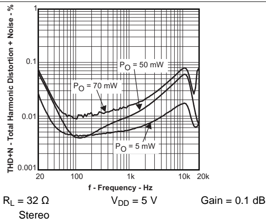
Figure 16. Total Harmonic Distortion + Noise vs Frequency
