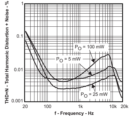
R_L = 32 \Omega BTL V_{DD} = 2.5 V Gain = 6.1 dB
