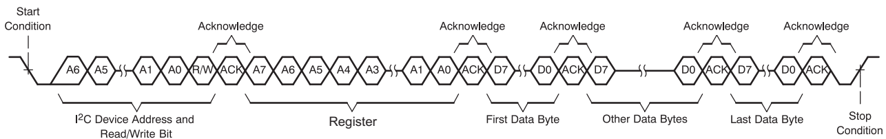
Figure 37. Multiple-Byte Write Transfer
