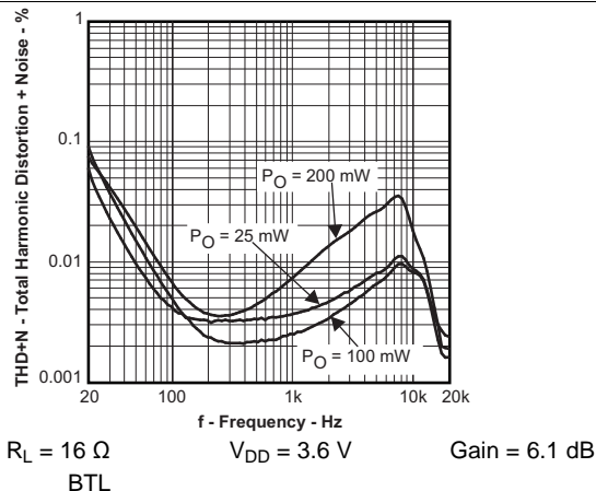
Figure 18. Total Harmonic Distortion + Noise vs Frequency
