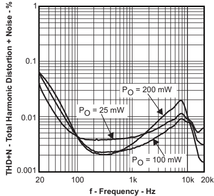
R_L = 16 \Omega BTL V_{DD} = 5 V Gain = 6.1 dB
