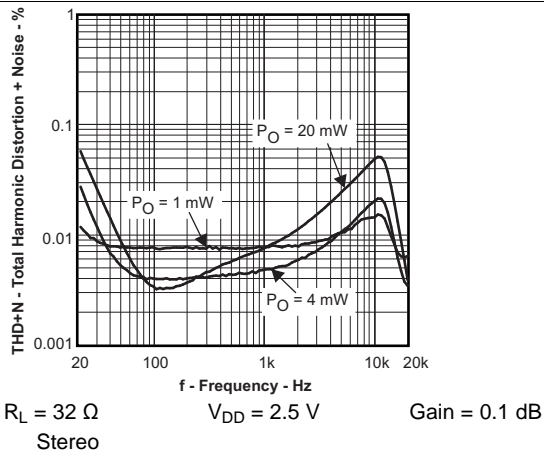
Figure 13. Total Harmonic Distortion + Noise vs Frequency
