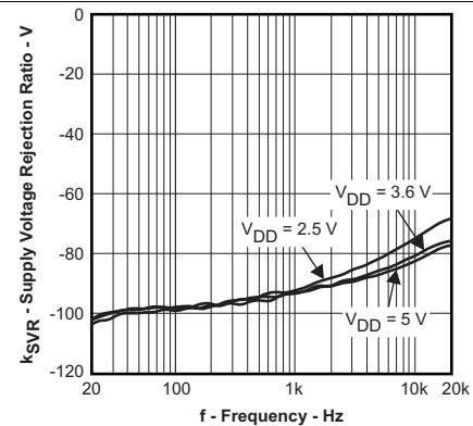
R_L = 32 \Omega Stereo C_p = 1 \mu F Gain = 0.1 dB
