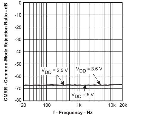
R_L = 16 \Omega C_l = 2.2 \mu F Gain = 0.1 dB Stereo
