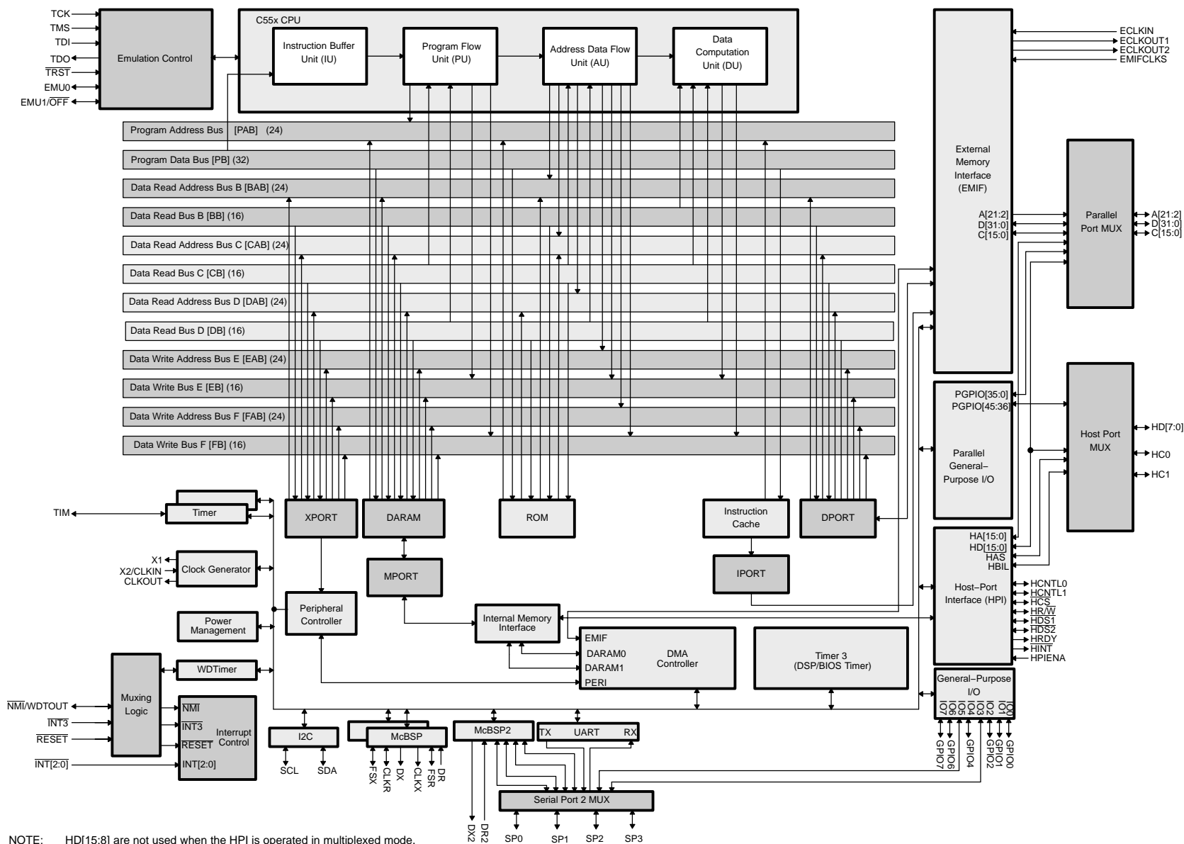
Figure 3–1. TMS320VC5502 Functional Block Diagram
