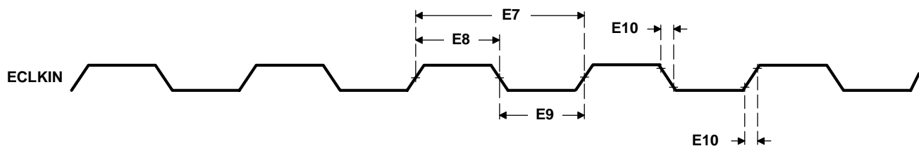
Figure 6–5. ECLKIN Timings for EMIF
