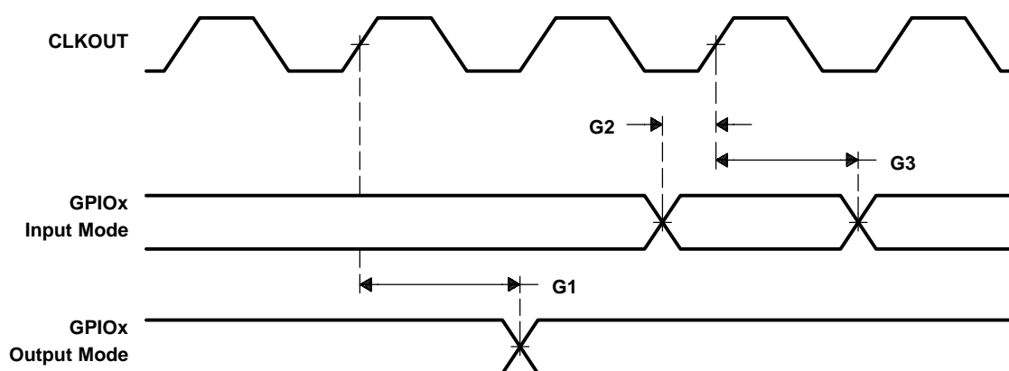
Figure 6–26. General-Purpose Input/Output (GPIO x ) Signal Timings
