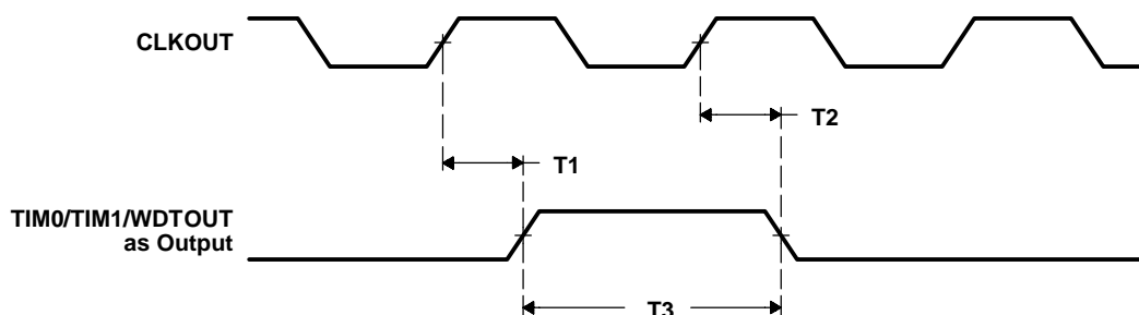
Figure 6–29. TIM0/TIM1/WDTOUT Timings When Configured as Timer Output Pins
