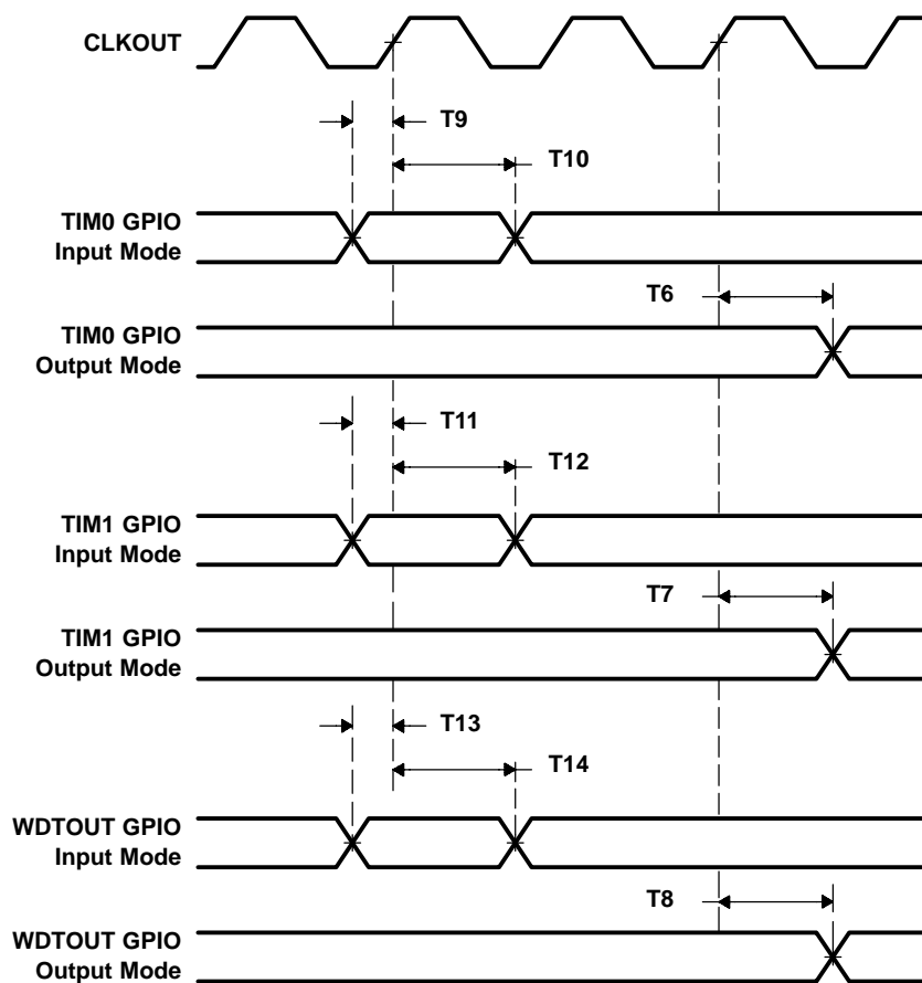
Figure 6–30. TIM0/TIM1/WDTOUT General-Purpose I/O Timings
