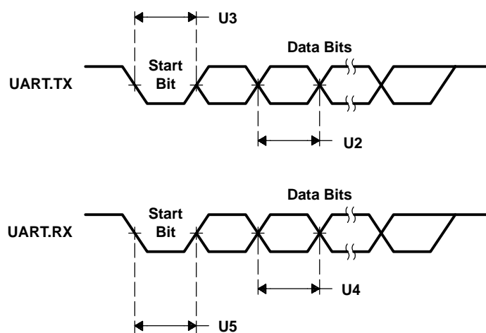
Figure 6–49. UART Timings
