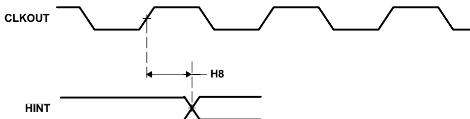
Figure 6–44. HINT Timings
