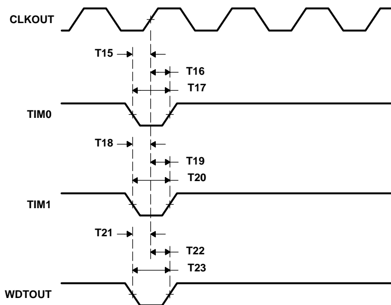
Figure 6–31. TIM0/TIM1/WDTOUT Interrupt Timings
