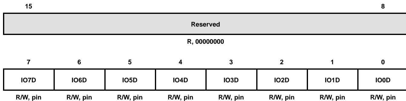
Figure 3–33. GPIO Data Register Layout (0x3401)
