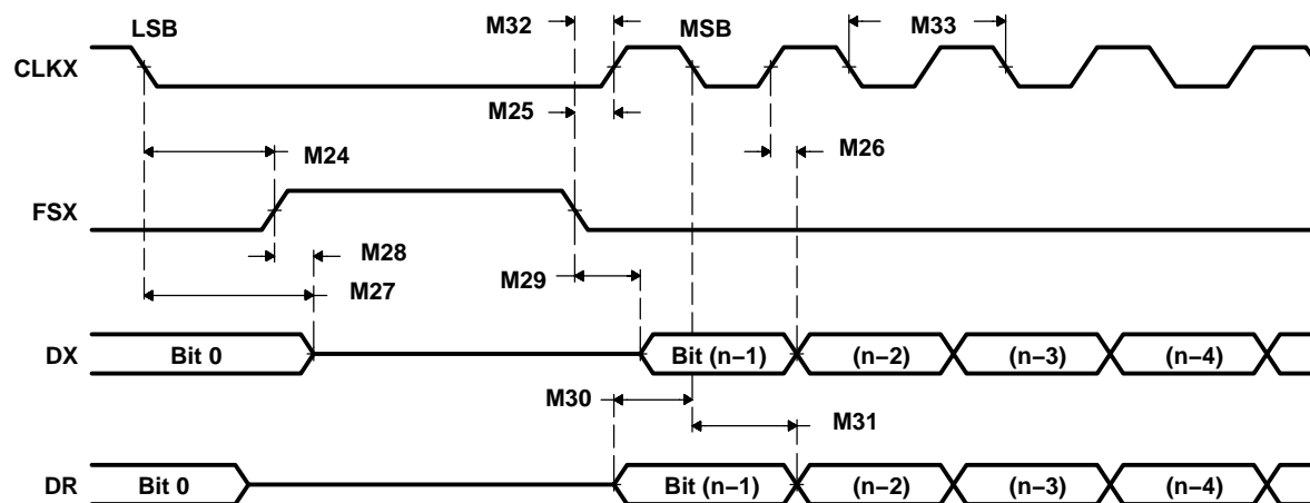
Figure 6–35. McBSP Timings as SPI Master or Slave: CLKSTP = 10b, CLKXP = 0
