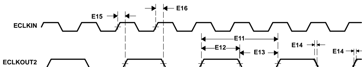
Figure 6–7. ECLKOUT2 Timings for EMIF Module
