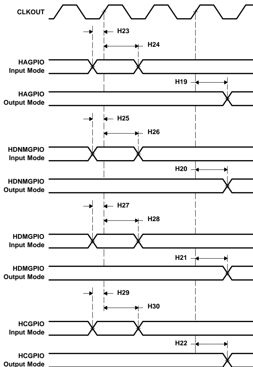
Figure 6–45. HPI General-Purpose I/O Timings
