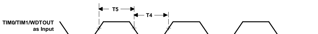
Figure 6–28. TIM0/TIM1/WDTOUT Timings When Configured as Timer Input Pins
