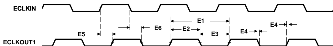
Figure 6–6. ECLKOUT1 Timings for EMIF Module
