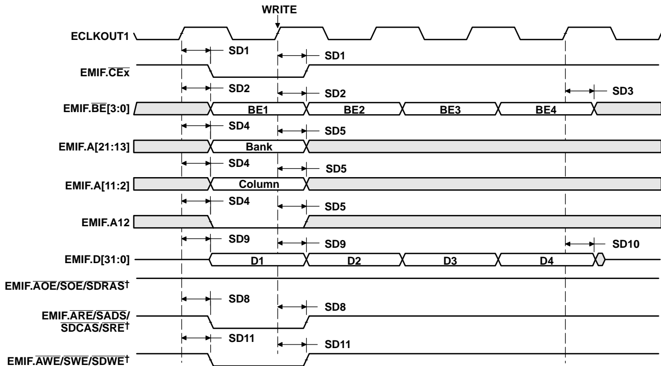
Figure 6–13. SDRAM Read Command (CAS Latency 3)
