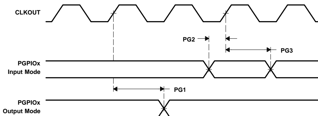
Figure 6–27. Parallel General-Purpose Input/Output (PGPIO x ) Signal Timings
