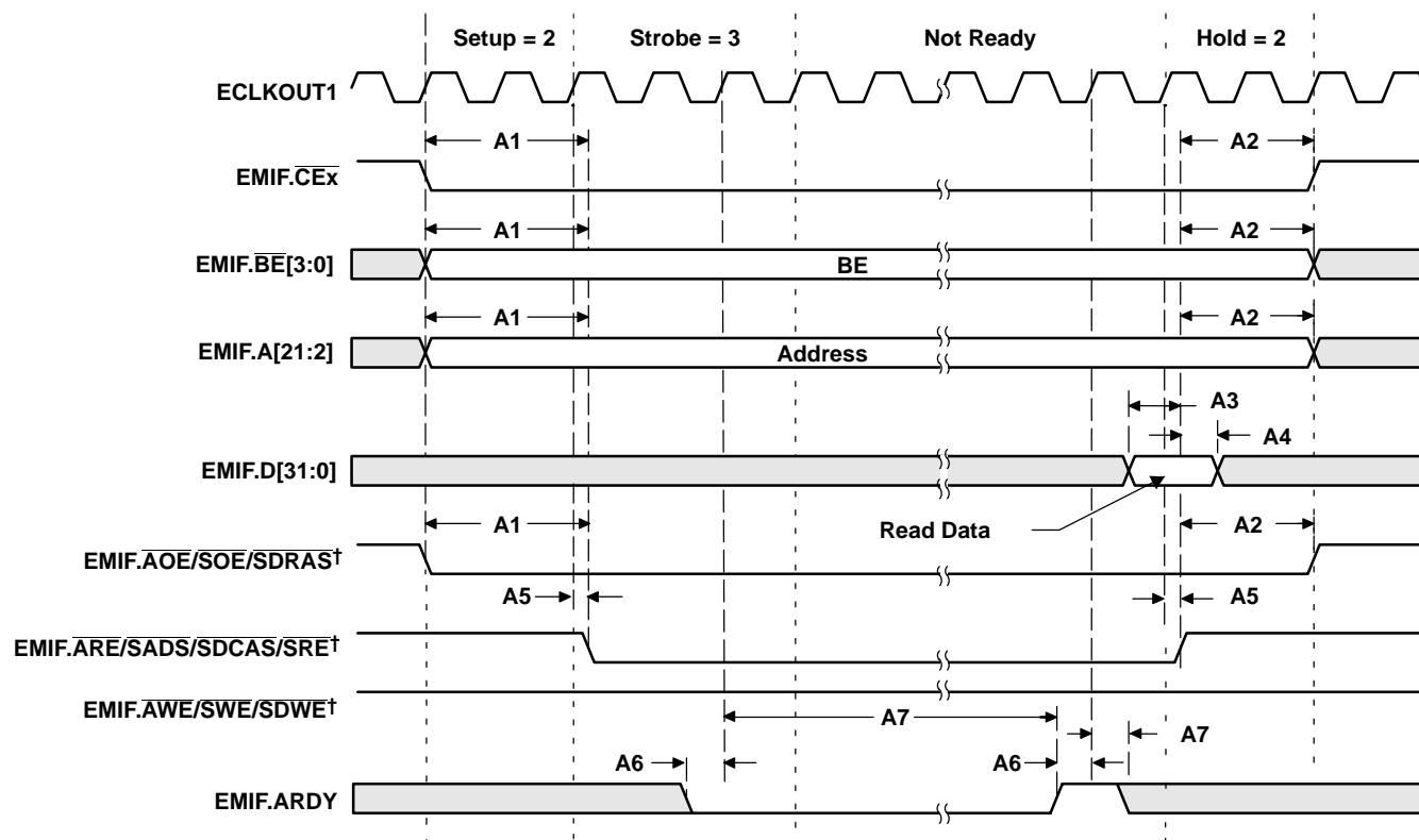
Figure 6–8. Asynchronous Memory Read Timings†
