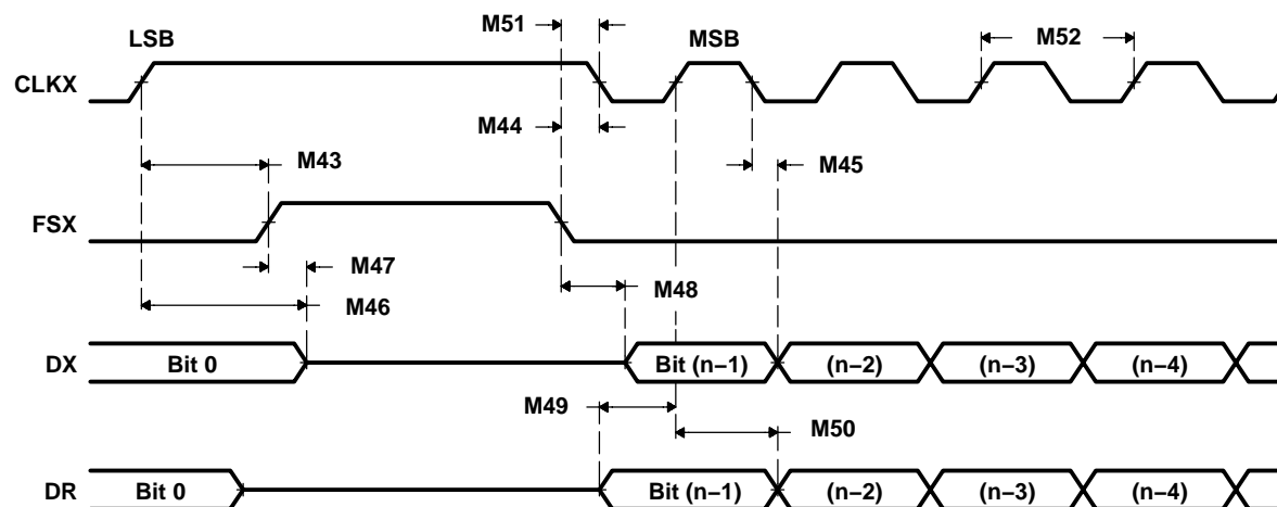
Figure 6–37. McBSP Timings as SPI Master or Slave: CLKSTP = 10b, CLKXP = 1
