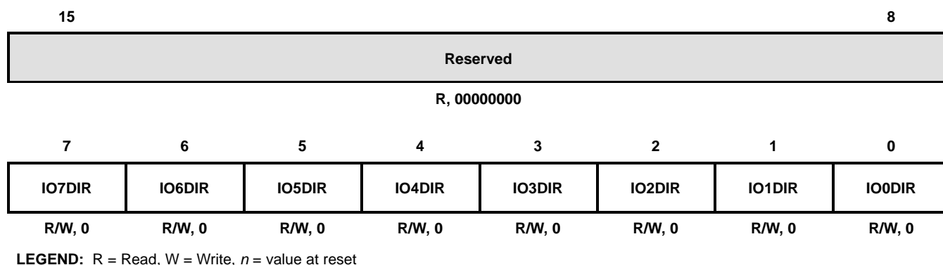
Figure 3–32. GPIO Direction Register Layout (0x3400)
