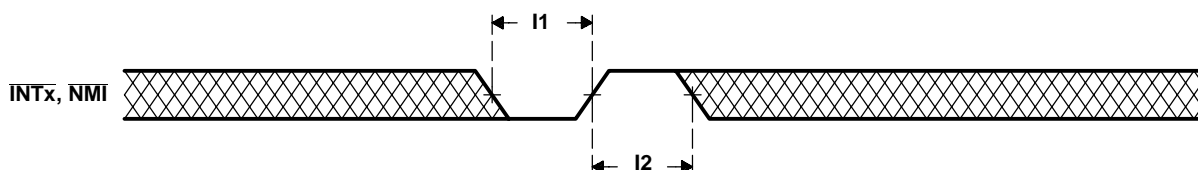
Figure 6–23. External Interrupt Timings
