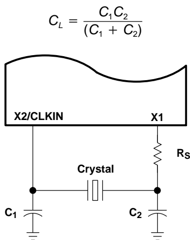
Figure 6–2. Internal System Oscillator With External Crystal
