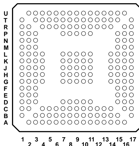
Figure 2–1. 201-Terminal GZZ Ball Grid Array (Bottom View)
