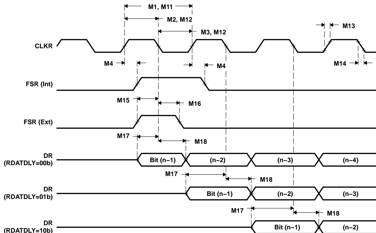
Figure 6-32. McBSP Receive Timings
