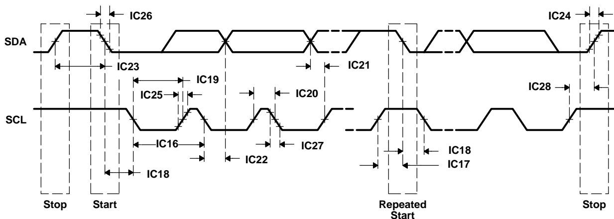
Figure 6–48. I 2 C Transmit Timings
