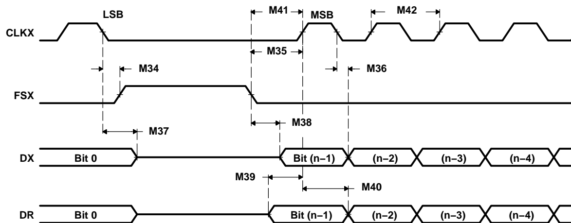
Figure 6–36. McBSP Timings as SPI Master or Slave: CLKSTP = 11b, CLKXP = 0
