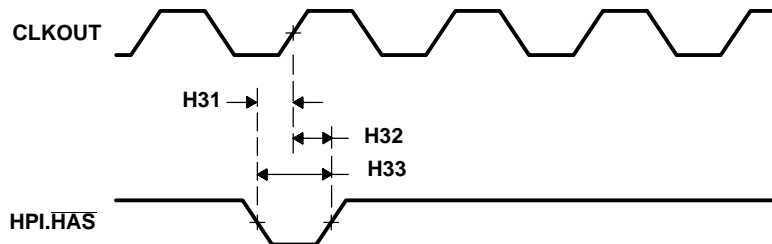
Figure 6–46. HPI.HAS Interrupt Timings
