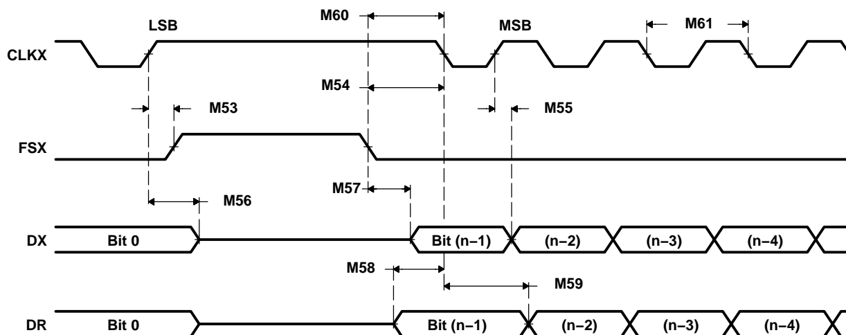
Figure 6–38. McBSP Timings as SPI Master or Slave: CLKSTP = 11b, CLKXP = 1
