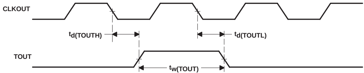
Figure 20. TOUT Timing
