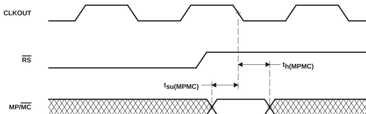
Figure 17. MP/MC Timing
