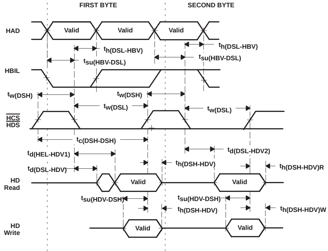
Figure 29. Read/Write Access Timings Without HRDY or \overline{HAS}
