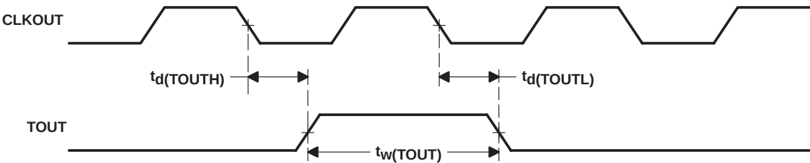
Figure 20. TOUT Timing
