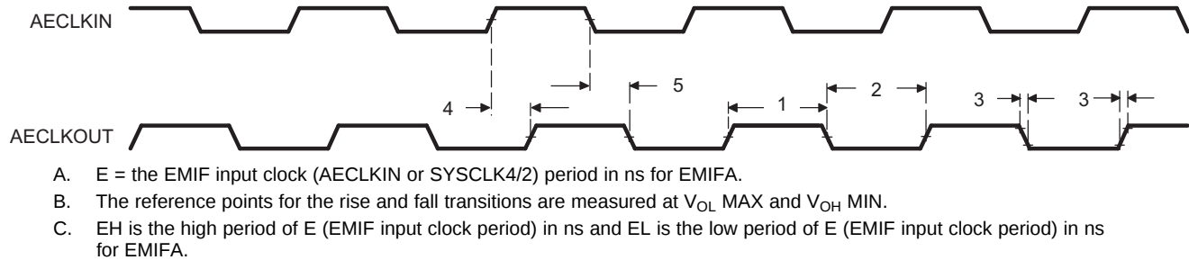
Figure 6-20. AECLKOUT Timing for the EMIFA Module
