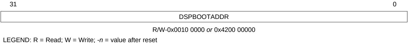
Figure 3-5. DSPBOOTADDR Register— 0x01C4 0008
