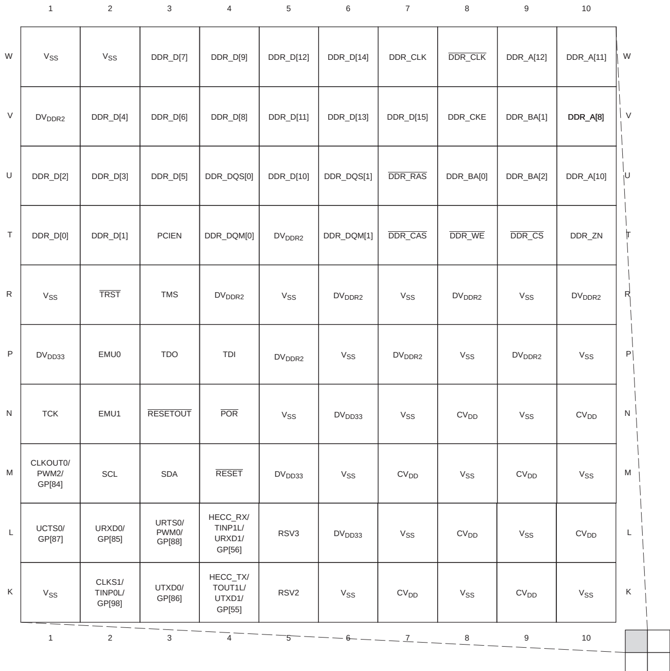
Figure 2-2. ZWT Pin Map [Quadrant A]
