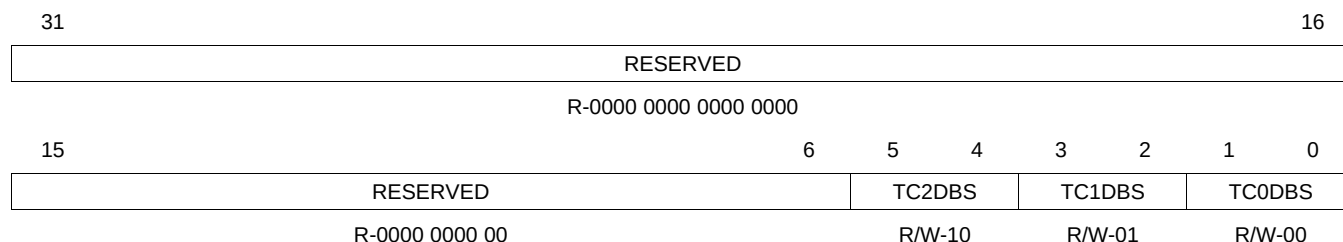
Figure 3-10. EDMA TC Configuration Register— 0x01C4 0088
