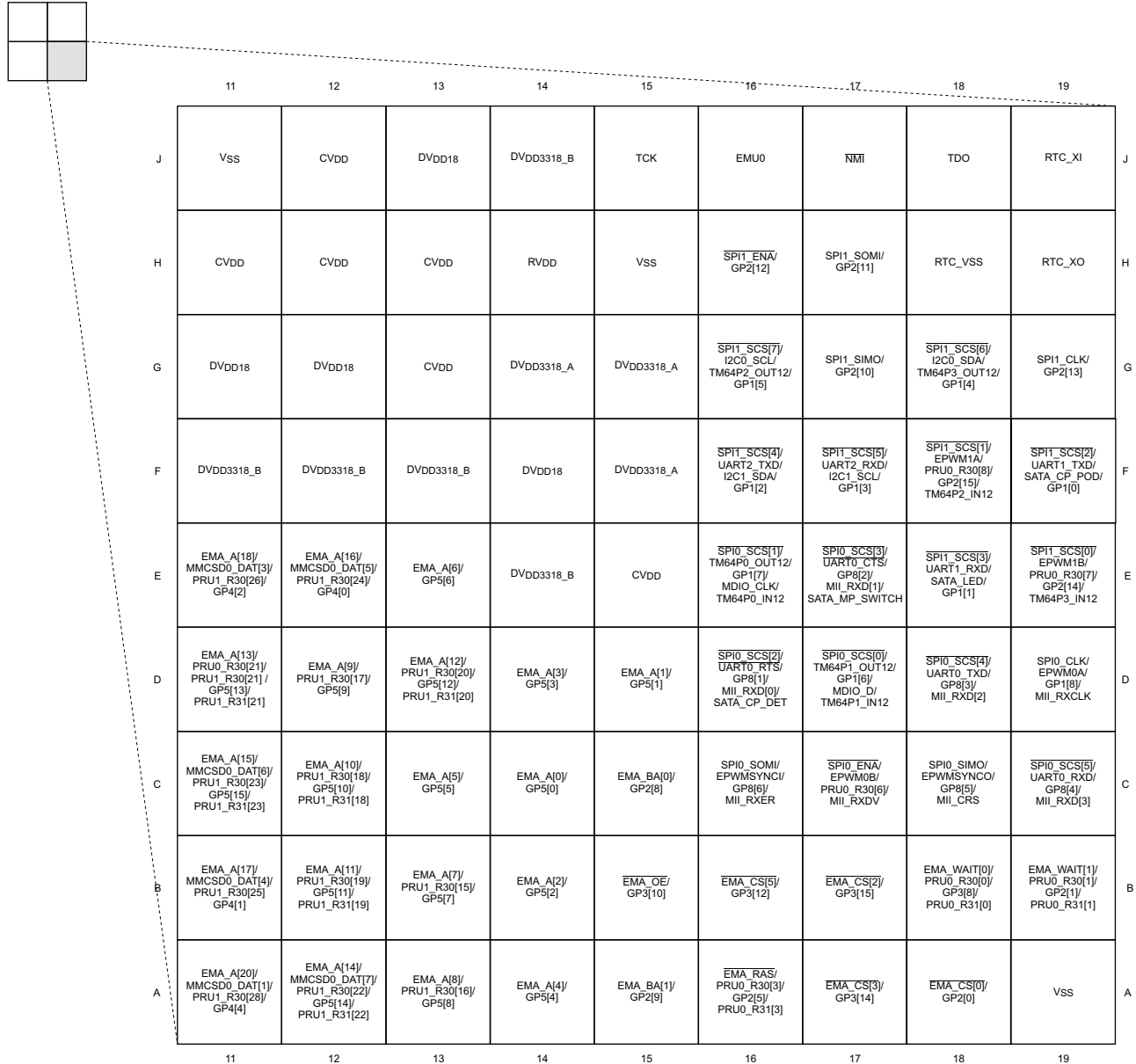
Figure 2-5. Pin Map (Quad C)
