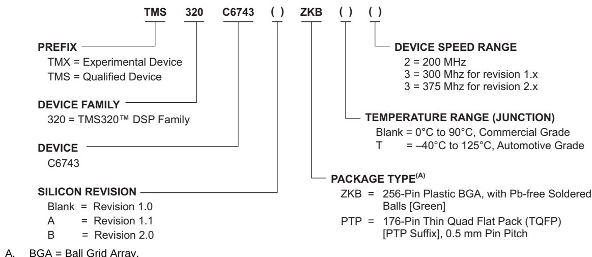
Figure 6-1. Device Nomenclature
