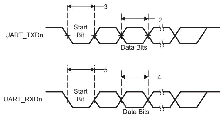
Figure 5-48. UART Transmit/Receive Timing
