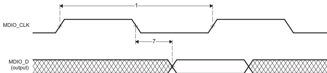
Figure 5-28. MDIO Output Timing
