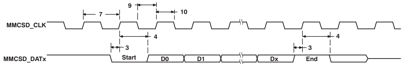
Figure 5-25. MMC/SD Host Read and Card CRC Status Timing
