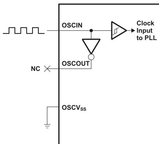
Figure 5-7. External 1.2V Clock Source
