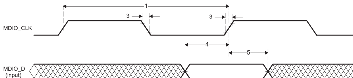
Figure 5-27. MDIO Input Timing
