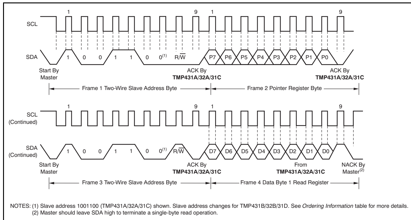
Figure 18. Two-Wire Timing Diagram for Single-Byte Read Format
