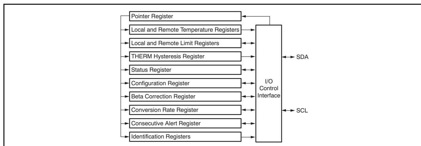
Figure 15. Internal Register Structure
