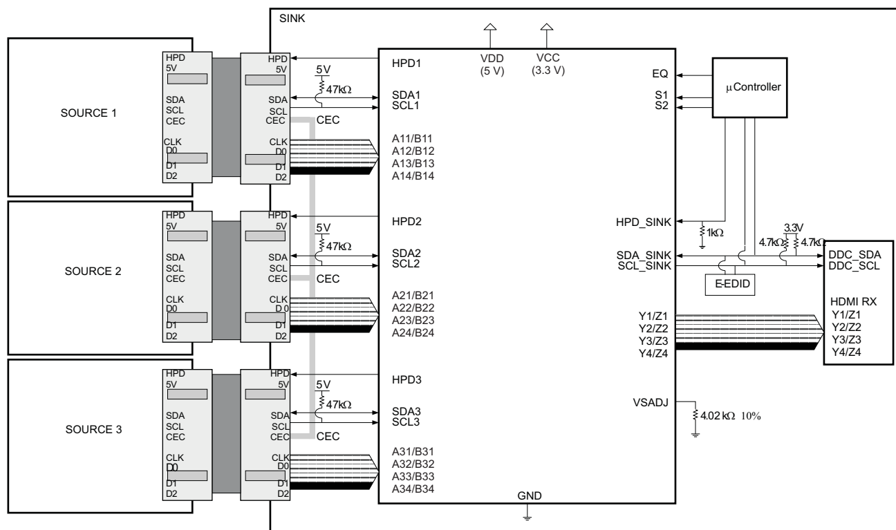
Figure 34. Three-Port HDMI-Enabled DTV With TMD5361 – CEC Commands Passing Through
