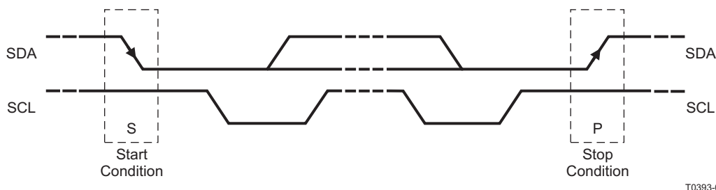
Figure 36. I²C Start and Stop Conditions
