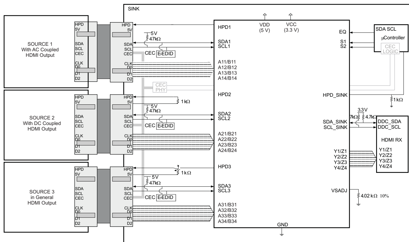
Figure 35. Three-Port HDMI-Enabled DTV With TMDS361 – CEC Commands Active
