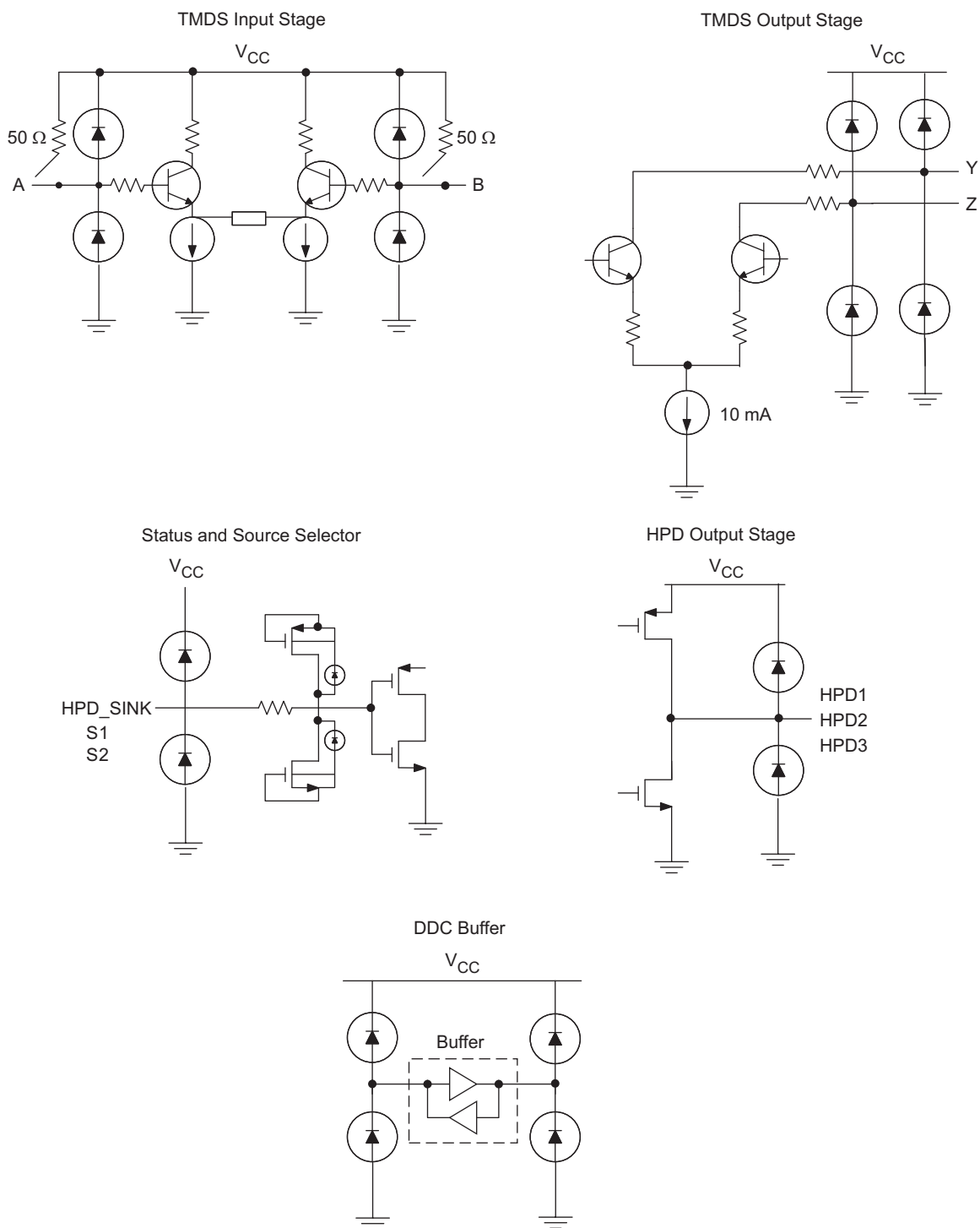
EQUIVALENT INPUT AND OUTPUT SCHEMATIC DIAGRAMS
