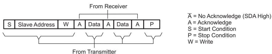
Figure 40. I²C Write Cycle
