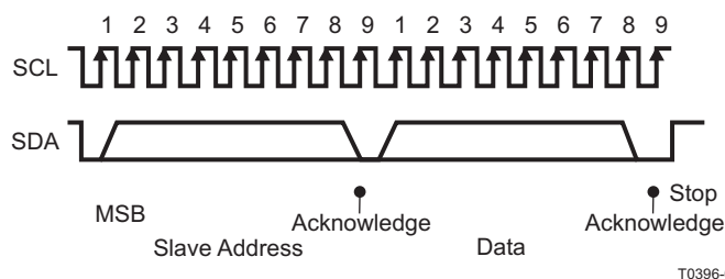
Figure 39. I²C Address, Data Cycle(s), and Stop
