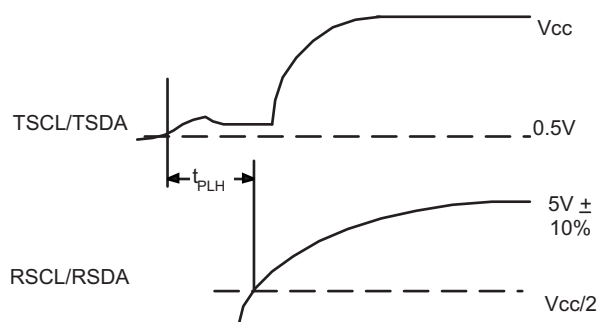
Figure 29. Waveform of Driver T Turning Off
