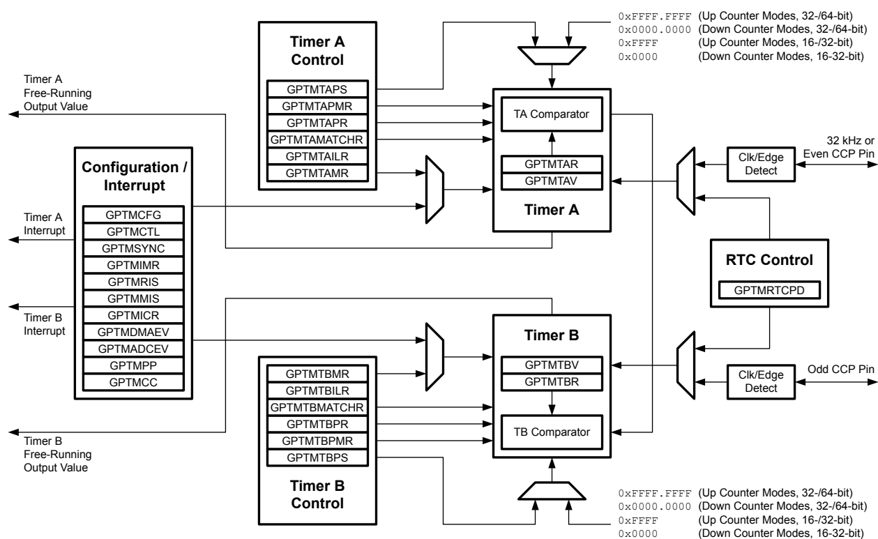
Figure 16-1. GPTM Module Block Diagram
