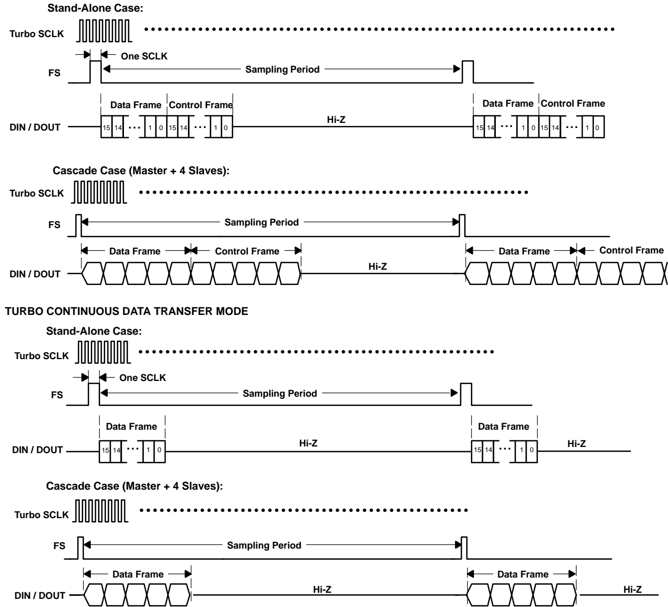
Figure 3–18. Timing Diagram for Turbo Operation
