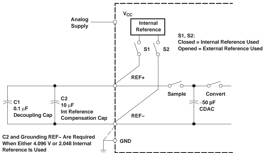
Figure 54. Reference Block
