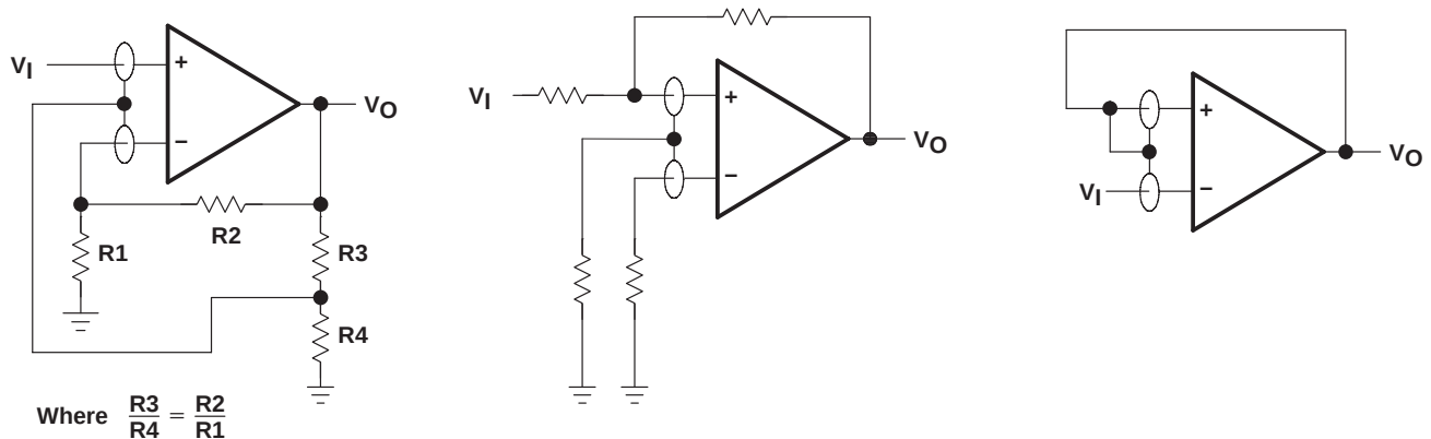
Figure 44. Use of Guard Rings
