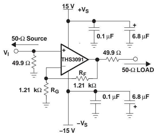
Figure 59. Wideband, Noninverting Gain Configuration
