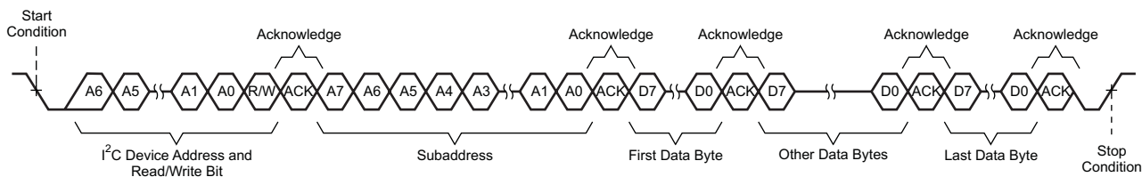
Figure 41. Multiple-Byte Write Transfer
