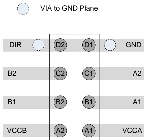
Figure 12. Layout Example for YZP Package
