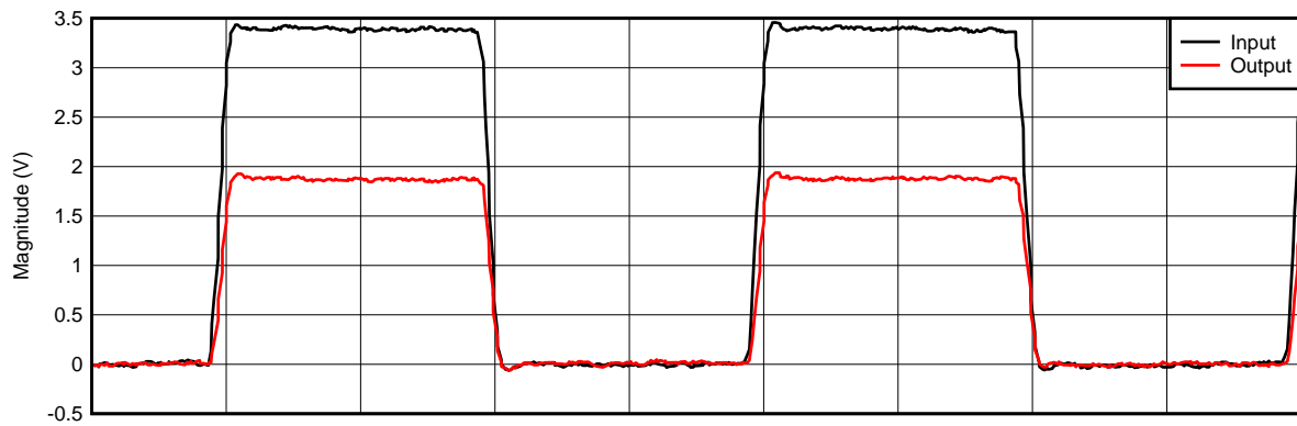
Figure 11. 3.3 V to 1.8 V Level-Shifting With 1-MHz Square Wave
