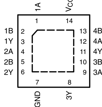
SN74AHC08 . . . RGY PACKAGE (TOP VIEW)
