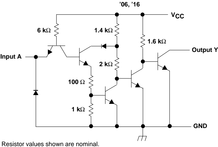
schematic (each buffer/driver)
