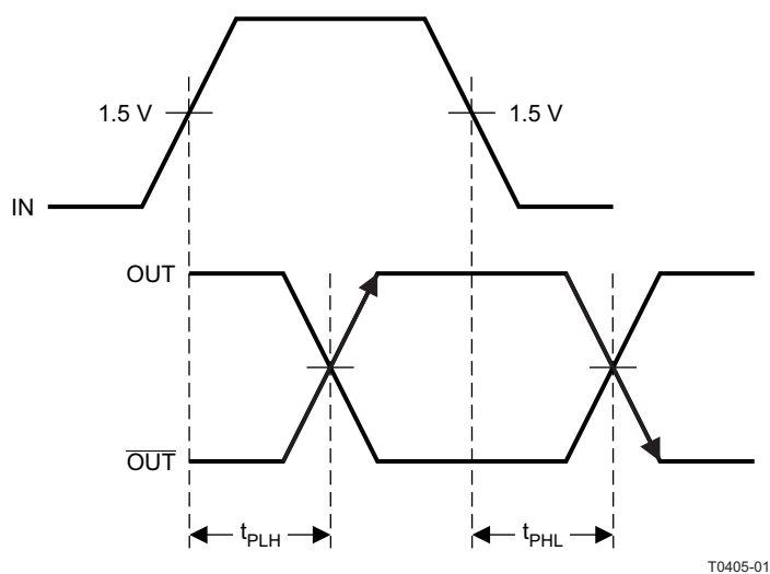
Figure 2. Output Propagation Delay
