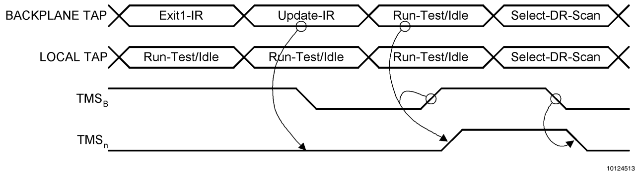
FIGURE 10. Local Scan Port Synchronization from Parked-RTI State
