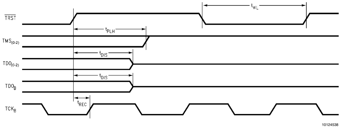
FIGURE 16. Reset Waveforms
