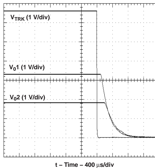
Figure 15. Simultaneous Power Down with Auto-Track Control
