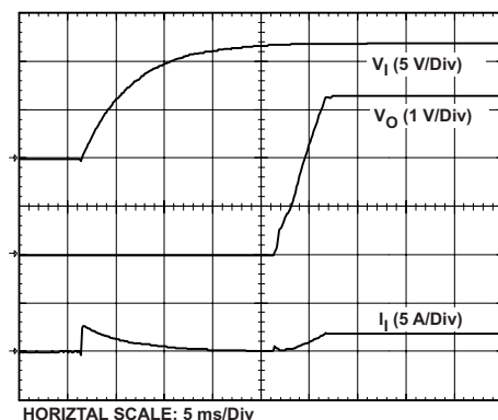
Figure 10. Power-Up Waveforms
