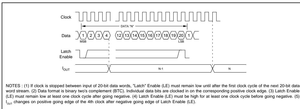
FIGURE 2. Timing Diagram.
