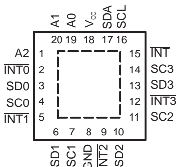
RGW PACKAGE (TOP VIEW)
