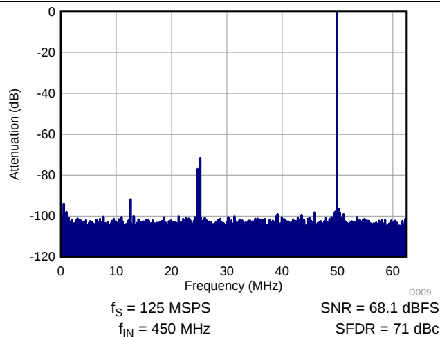
Figure 65. Performance FFT at 450 MHz (High Input Frequency)
