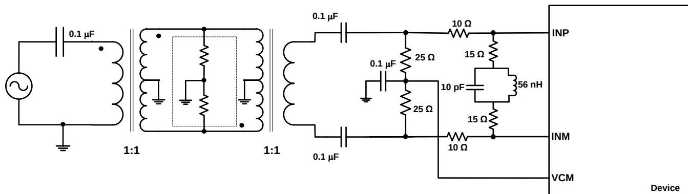
Figure 62. Driving Circuit for Mid-Range Input Frequencies ( 100 \text{ MHz} < f_{\text{IN}} < 230 \text{ MHz} )
