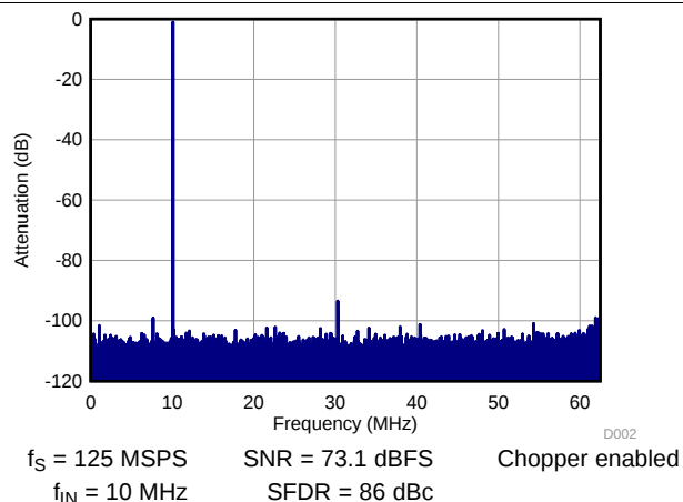
Figure 2. FFT with Dither Off
