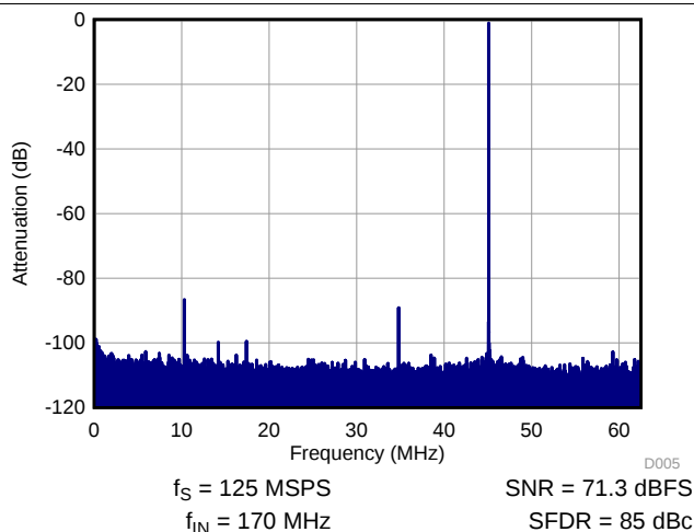
Figure 63. Performance FFT at 170 MHz (Mid Input Frequency)
