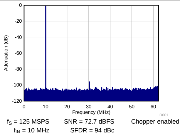
Figure 1. FFT with Dither On
