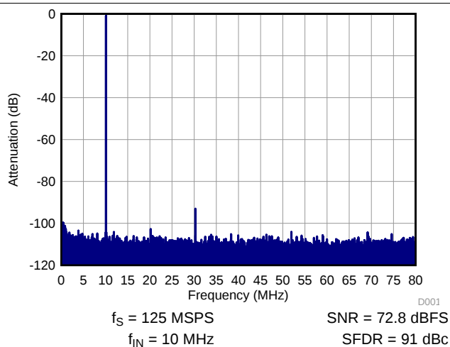
Figure 61. Performance FFT at 10 MHz (Low Input Frequency)
