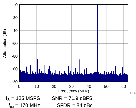
Figure 6. FFT with Dither Off
