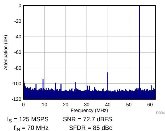
Figure 4. FFT with Dither Off
