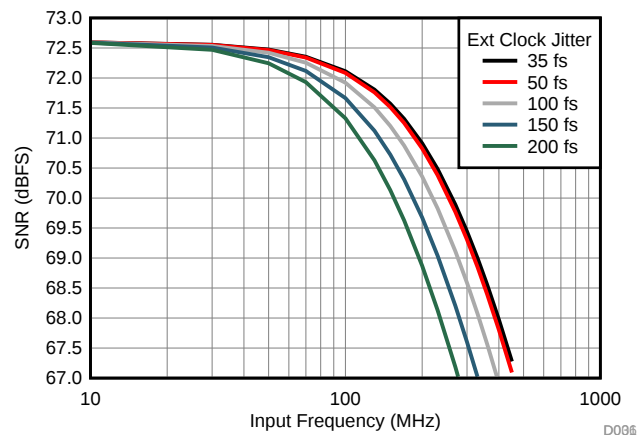
Figure 22. SNR vs Frequency for Different Clock Jitter
