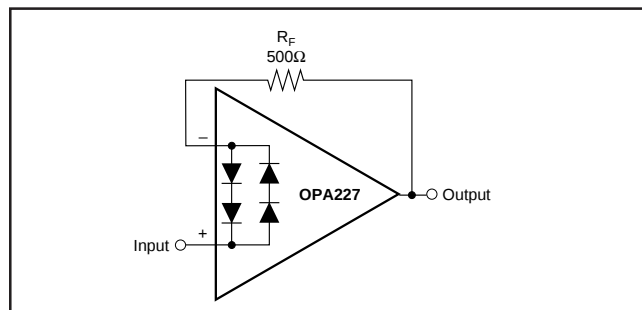
FIGURE 2. Pulsed Operation.
