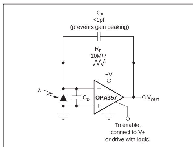
Figure 9. Transimpedance Amplifier
