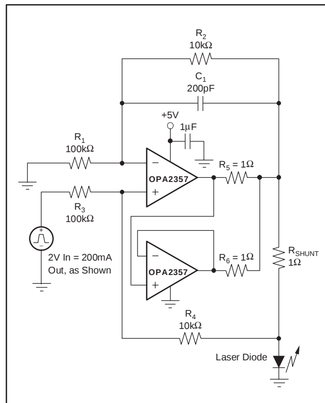
Figure 3. Parallel Operation
