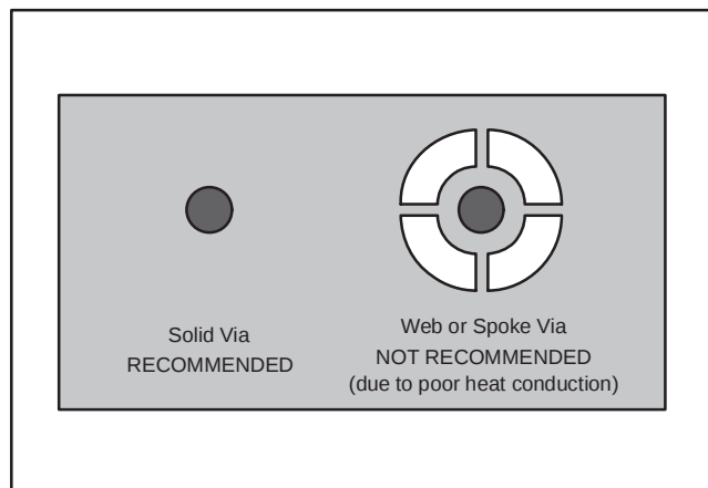
Figure 12. Via Connection
