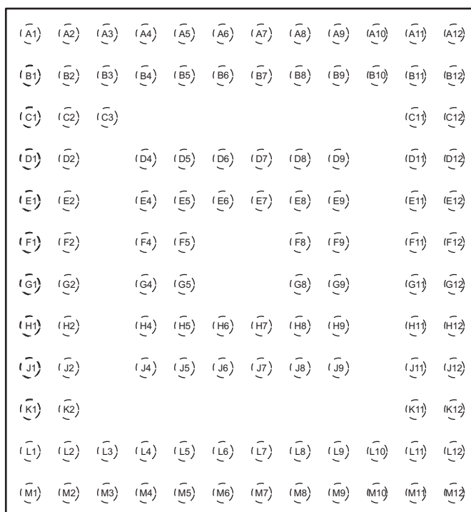
ZQW PACKAGE (TOP VIEW)
