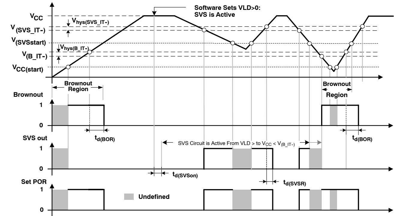
Figure 9. SVS Reset (SVSR) vs Supply Voltage
