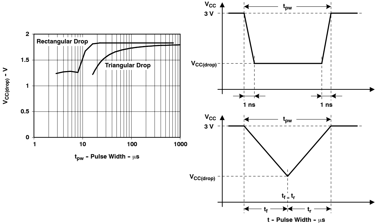
Figure 10. V_{CC(drop)} With a Square Voltage Drop and a Triangular Voltage Drop to Generate an SVS Signal
