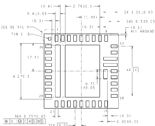
Leadless Leadframe Package (NS Package Number LQA036A), (Bottom View)
