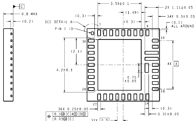
Leadless Leadframe Package (NS Package Number LQA036D), D Version (Bottom View)
