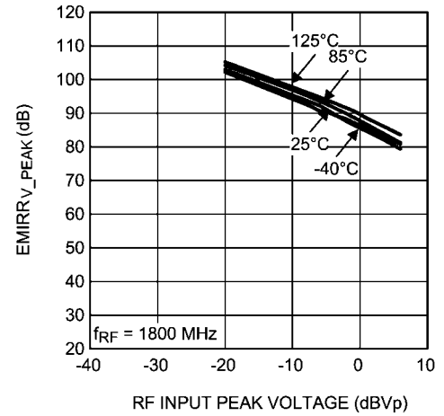
EMIRR IN+ vs. Power at 1800 MHz
