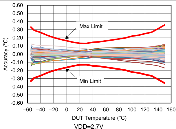
Figure 3. Temperature Accuracy
