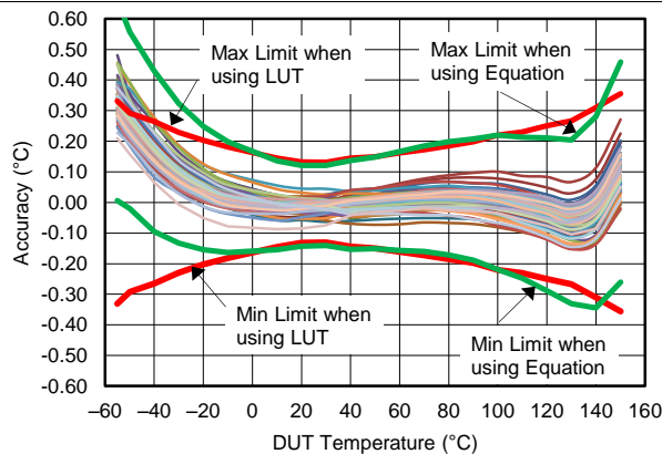
Figure 31. Using Second Order Transfer Function Best Fit -10°C to 110°C
