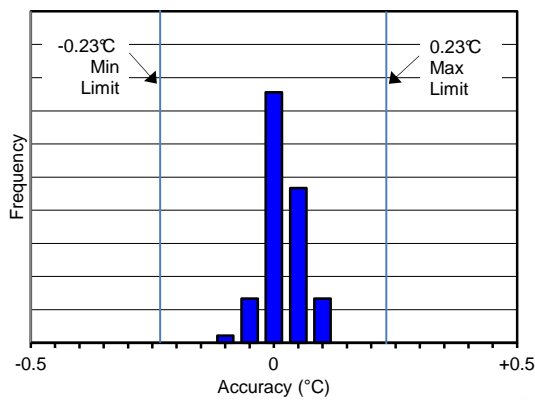
Figure 9. Accuracy Histogram at 50°C
