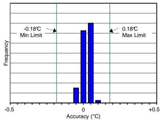
Figure 4. Accuracy Histogram at -55°C
