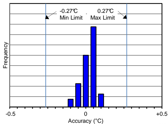
Figure 3. Temperature Accuracy
