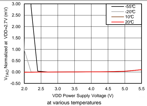
Figure 20. Line Regulation Temperature Variation: V_{TAO} vs Supply Voltage
