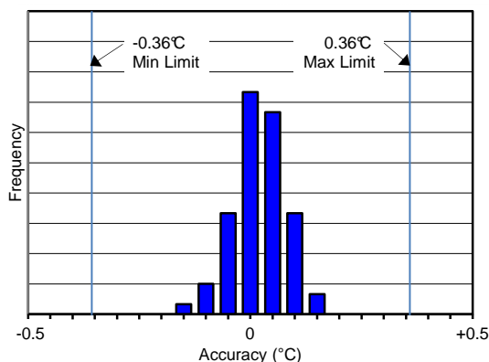
Figure 13. Accuracy Histogram at 150°C
