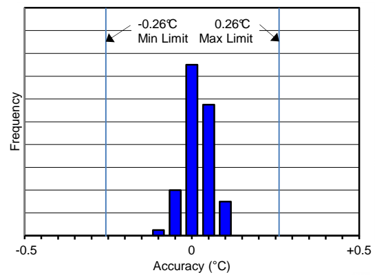
Figure 10. Accuracy Histogram at 90°C
