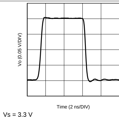
Figure 39. Large Signal Step Response
